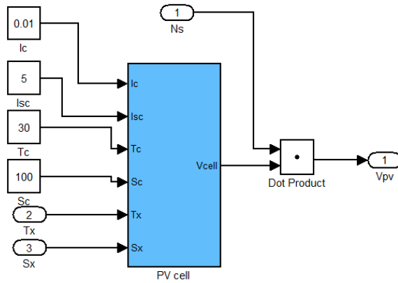
Fig-1.2.2: Modeling Stage 2
