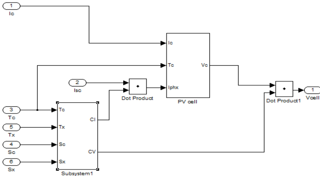
Fig-1.2.3: Modeling Stage 3
