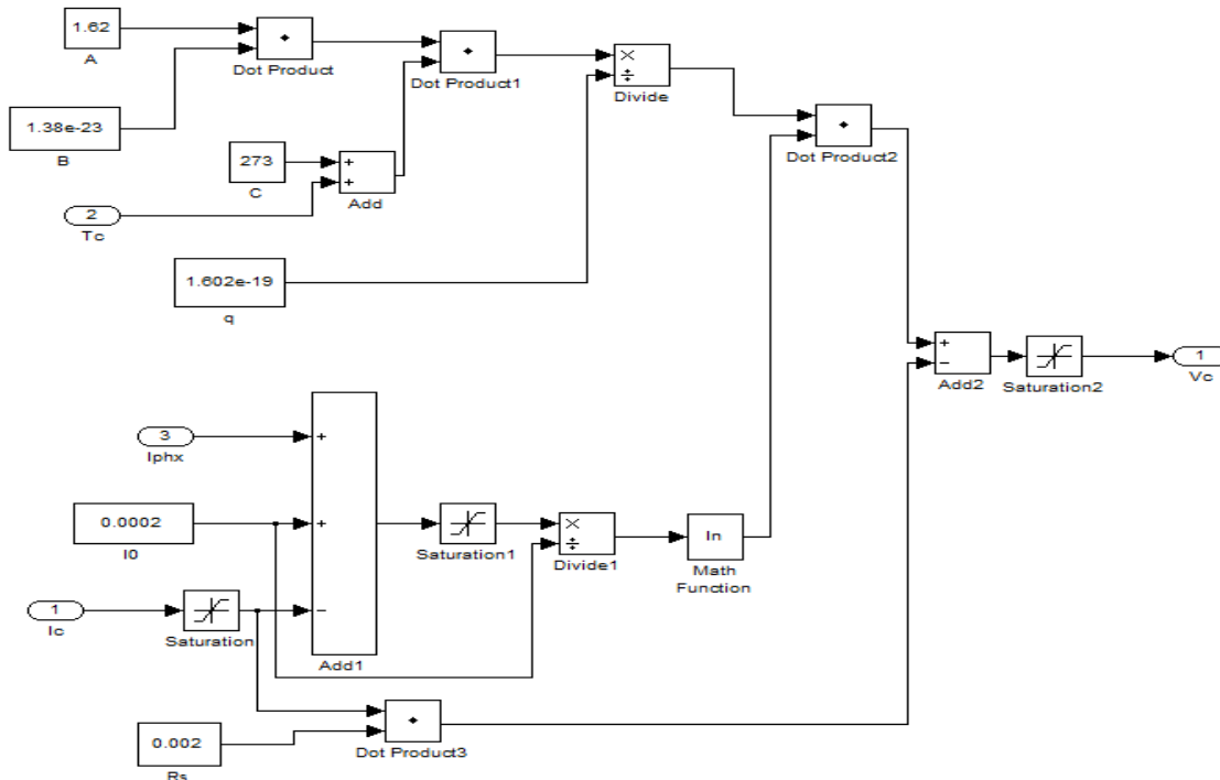
Fig-1.2.4: Mathematical Sub mask system of PV cell
