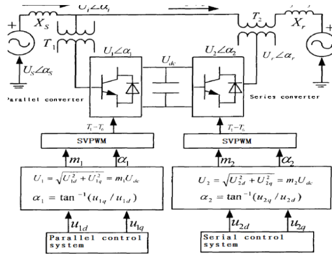
Fig -2: Basic Structure of UPFC connected to power system
