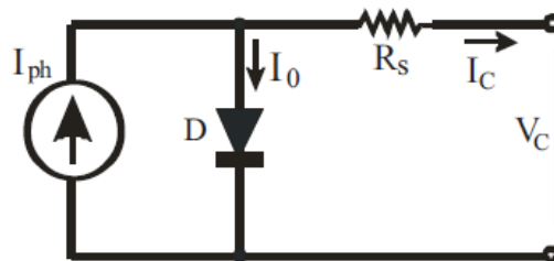
Fig-1: Simplified Circuit of Photovoltaic Cell
