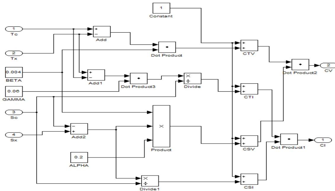
Fig-1.2.5: Mathematical Sub mask system of Subsystem 1
