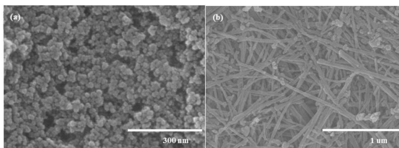
Figure 8:- FE-SEM images of TiO 2 nanoparticles and TNT films, (a) TiO 2 nanoparticles made by sol-gel method (b) TNT films made by hydrothermal method at 150°C for 12 h
