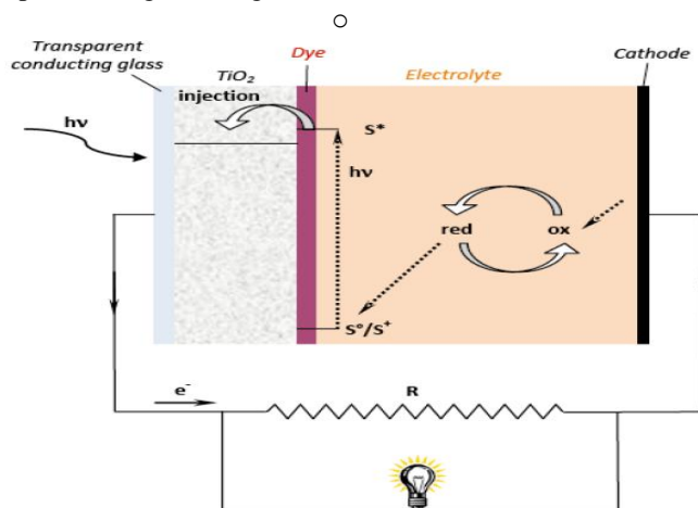
Fig1:- Schematic principle of a DSSC: photo excitation of the day (sensitizer, S) generates electrons which are injected into the conduction band of TiO 2 .
