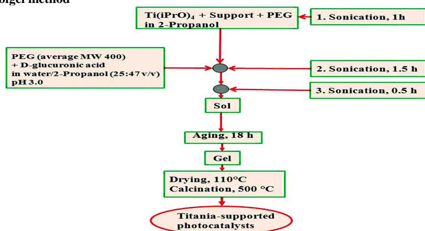
Figure 5:- Flow chart for preparation of TiO 2 nanoparticles using sol-gel method
