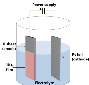
Figure 6:- Electrochemical Anodization technique
