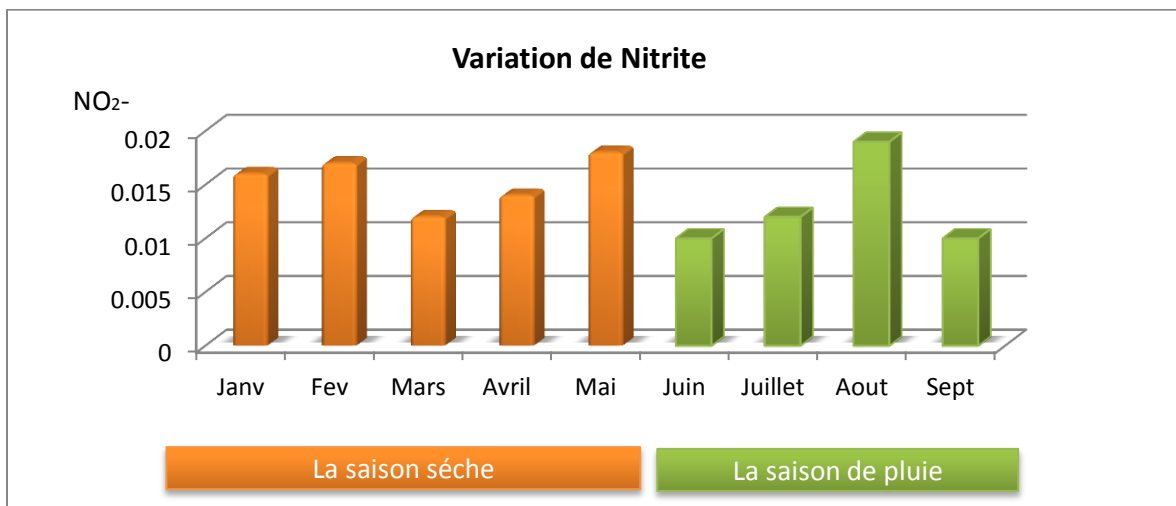
Figure 7: Variation du nitrite (NO 2 )
