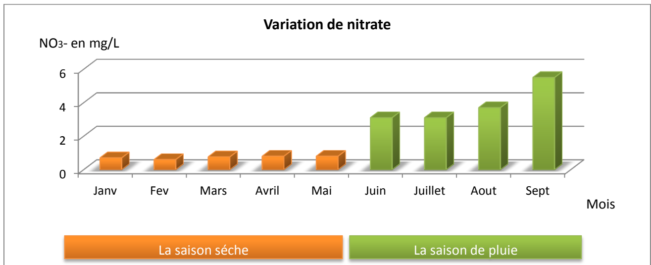
Figure 6:- Variation du nitrate (NO 3 )
