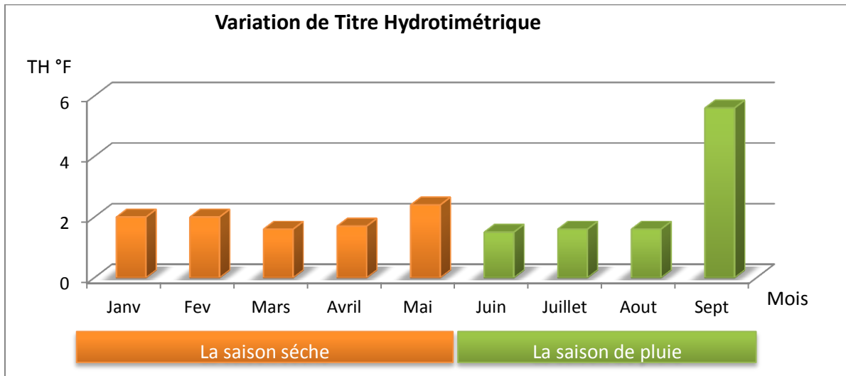
Figure 11:- Variation de TH
