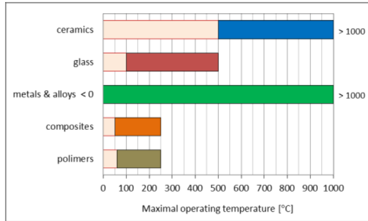
Figure 3:-Operating temperatures of materials
