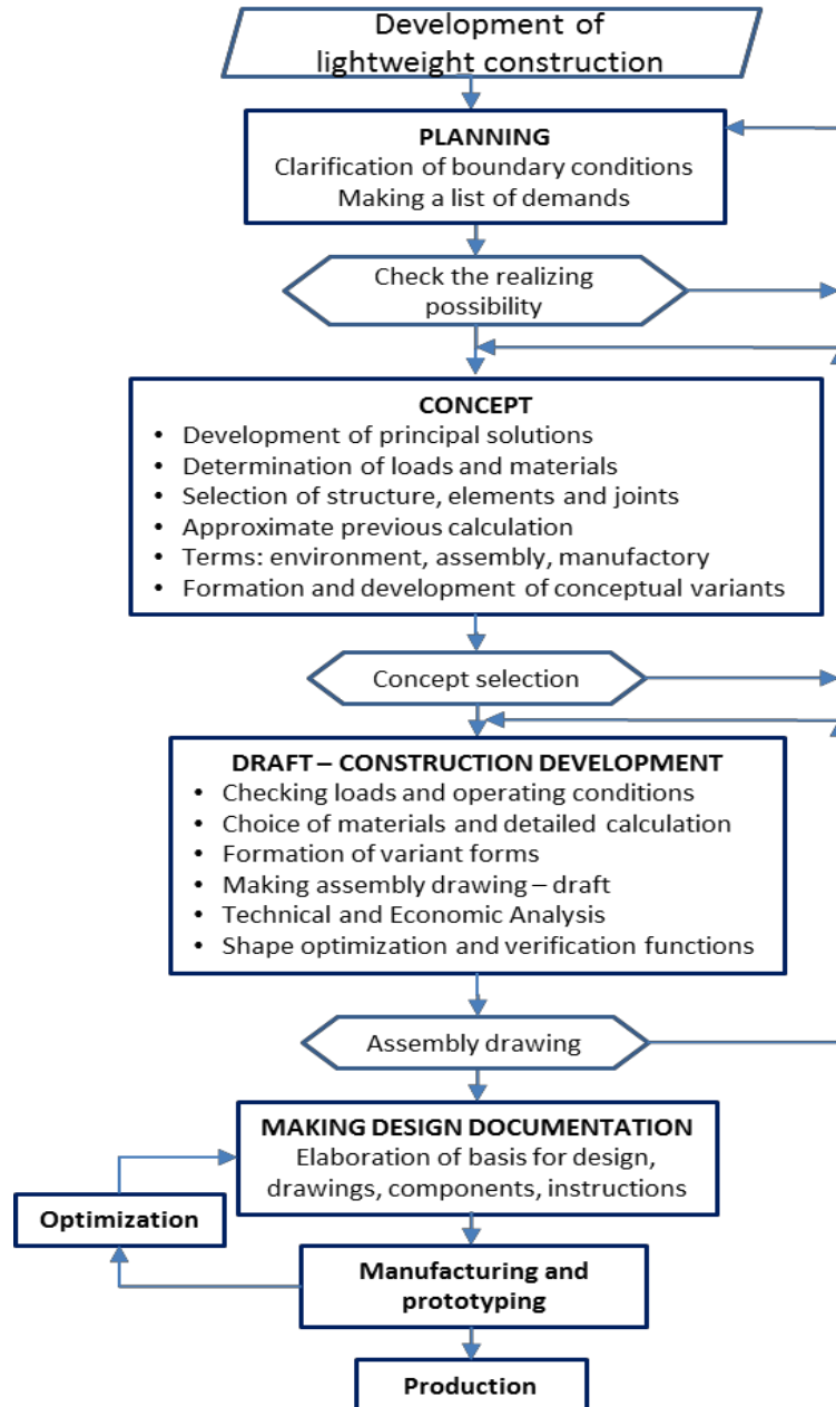
Figure 7:- Systematic approach in development of lightweight constructions [3-8,13]
