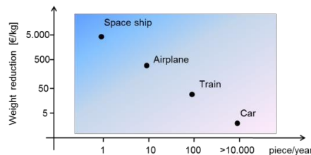
Figure 6:-Prices of lightweight constructions per kg of reduced weight [8]
