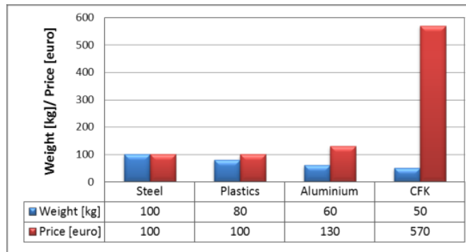
Figure 4:-Comparison of prices of materials used in lightweight design [6]
