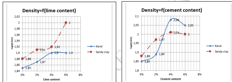
Figure 7. Dry density at Modified Proctor Optimum for blends, according to the binding agent's percentage
