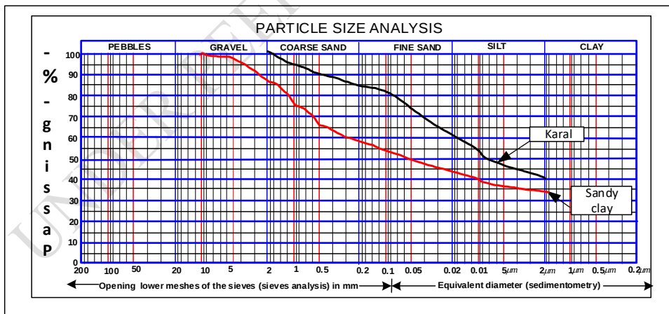
Figure 3. Granulometric analysis results.
