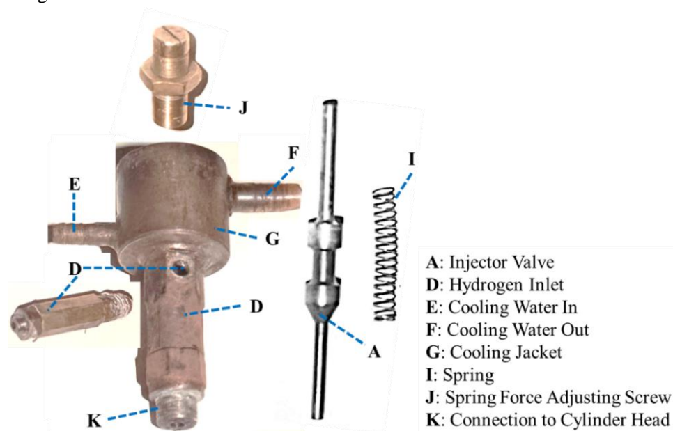
Figure 6. Mechanically Activated Gas Fuel Injector and main parts
