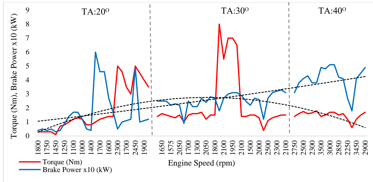
Figure 10. H 2 ICE Engine speed; Torque, Brake power
