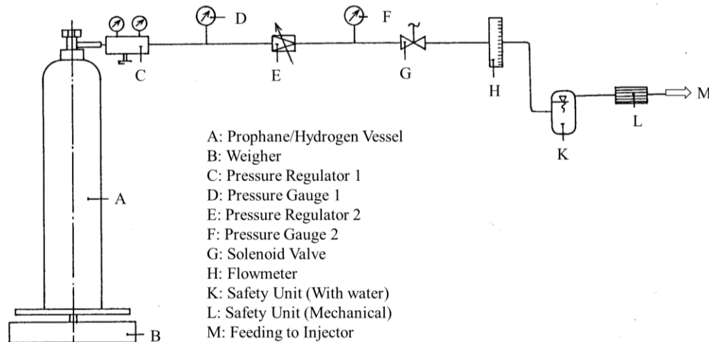
Figure 1. Experimental setup gas fuel supply equipment diagram and circuit equipment
