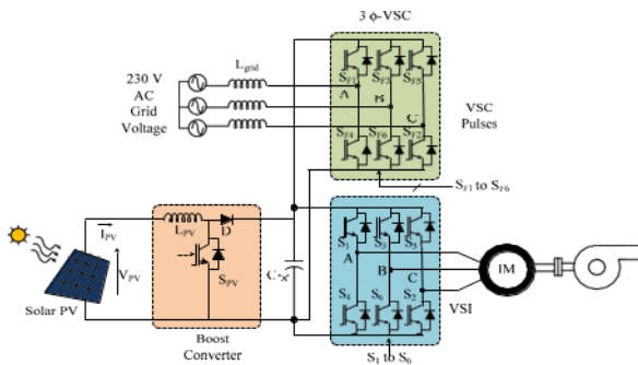
Figure 1. Configuring a bidirectional power flow capable smart solar water pumping system
