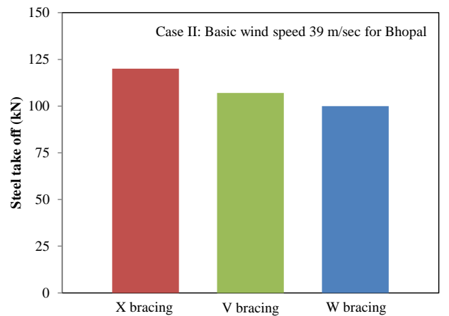
Figure 8 Steel take-off quantities for different bracing systems
