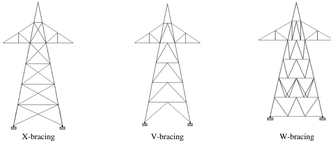
Figure 2 Tower with different bracing systems
