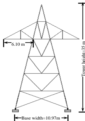
Figure 1 Transmission tower
