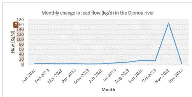
Figure 9 : Monthly change in lead flow (kg/d) in the Djonou river
