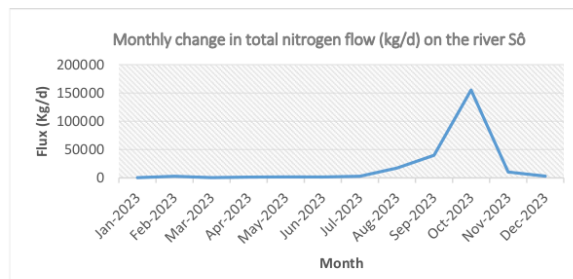
Figure 14: Monthly change in total nitrogen flow (kg/d) on the river Sô
