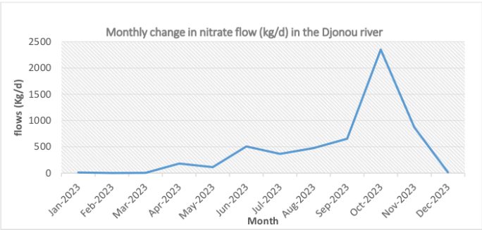
Figure 5 Monthly change in nitrate flow (kg/d) in the Djonou river
