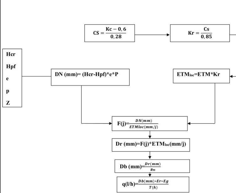
Figure 1: flowchart for determining basic parameters
