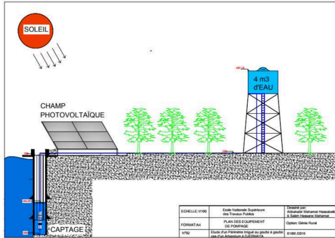
Figure 5: Pumping Station
