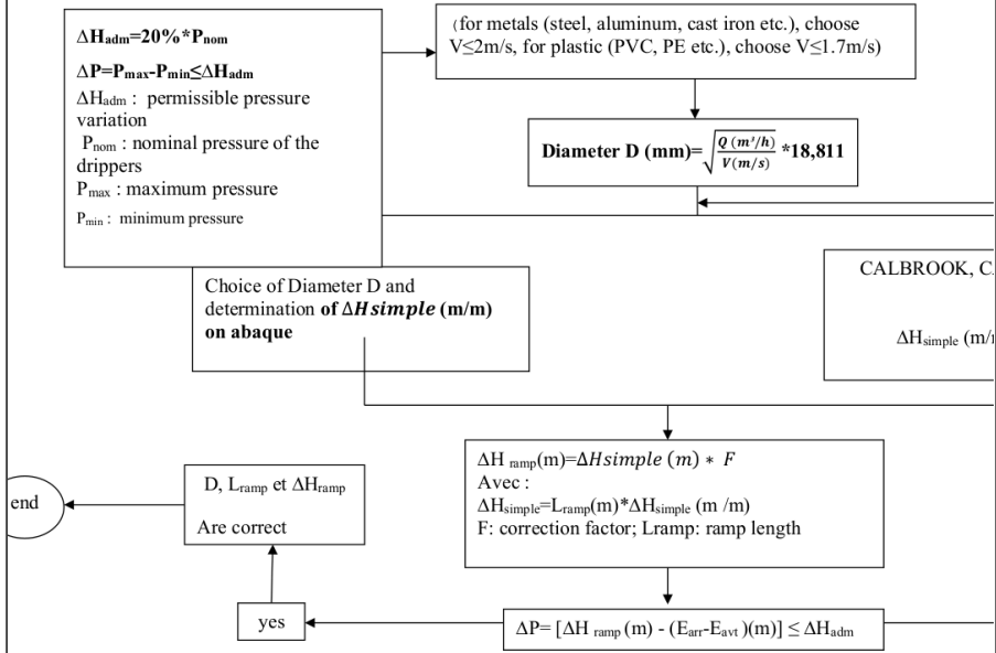
Figure 2 : tube sizing flowchart with en-route service
