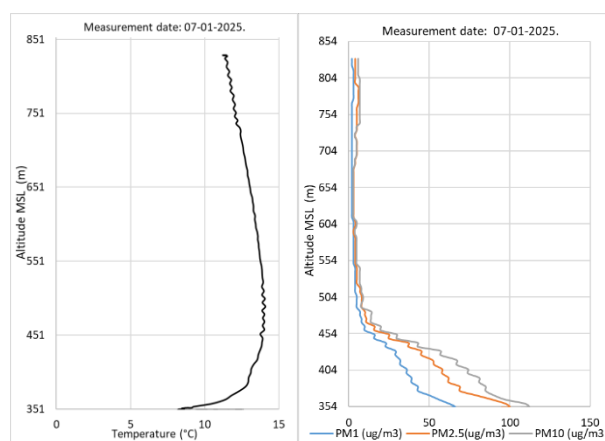
Figure 5. Vertical profiles of temperatures and PM concentrations at the Institute location
