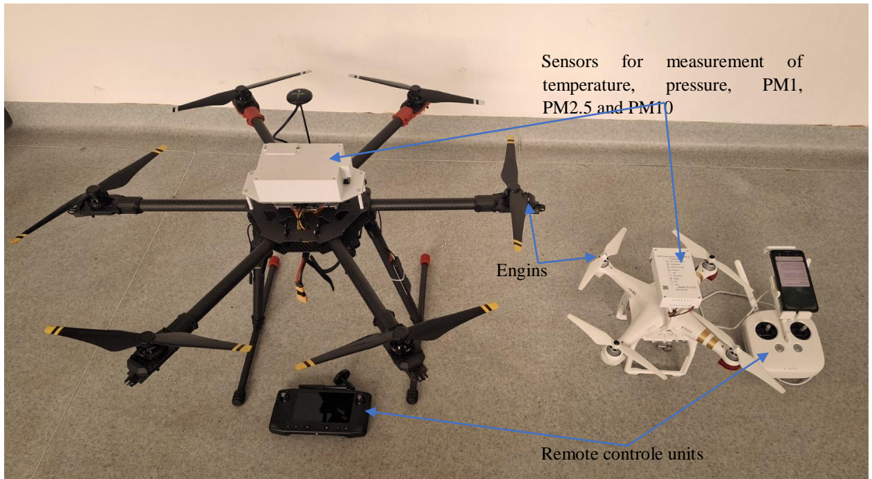
Figure 1. Unmanned aerial vehicles
