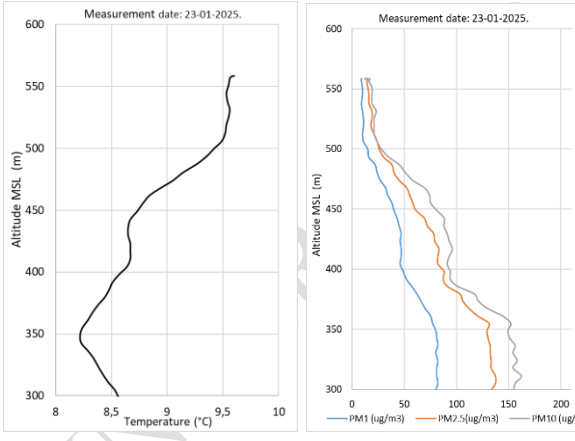
Figure 3. Vertical profiles of temperatures and PM concentrations at the Banlozi location
