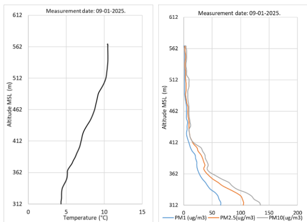
Figure 4. Vertical profiles of temperatures and PM concentrations at the Kamberovića polje location
