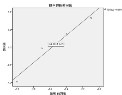
Figure 7.3 Fludioxonil EC 50 graph
