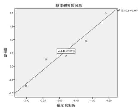
Figure 7.2 Fluazinam EC 50 graph
