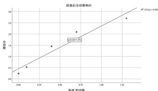
Figure 7.1 Tebuconazole EC 50 graph
