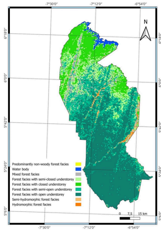
Figure IV: Spatial distribution of forest facies in the TNP
