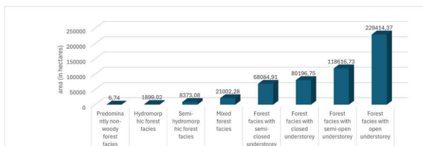
Figure 3: Graphical representation of the areas occupied by forest facies in the TNP
