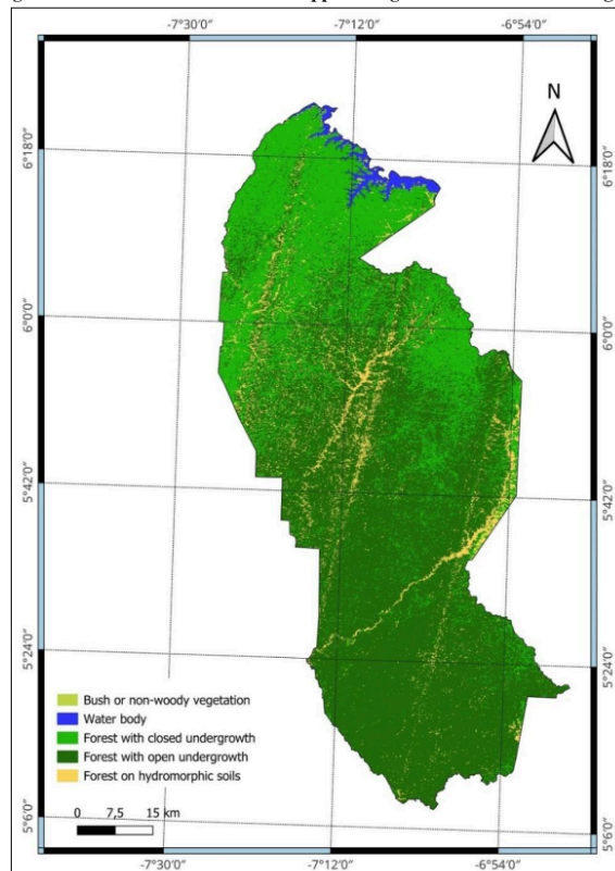
Figure 2: spatial distribution of forest formations mapped by image classification
