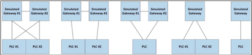
Figure 1 – Operation modes of the simulated gateway.
