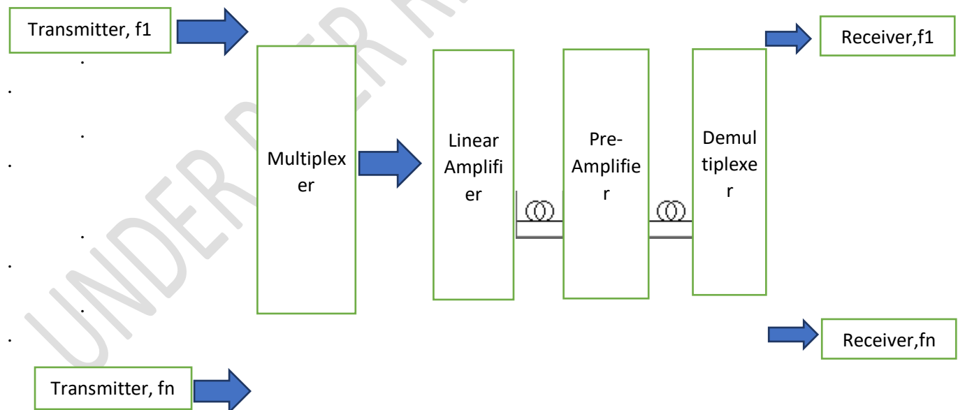
Figure 1: Diagram of the DWDM communication system model
