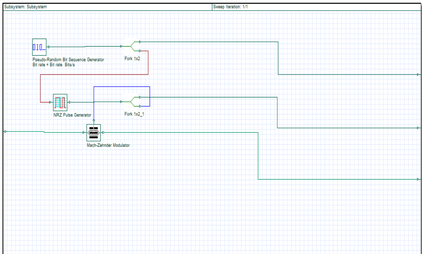
Figure 2:- Transmitter subsystem designed in Optisystem software
