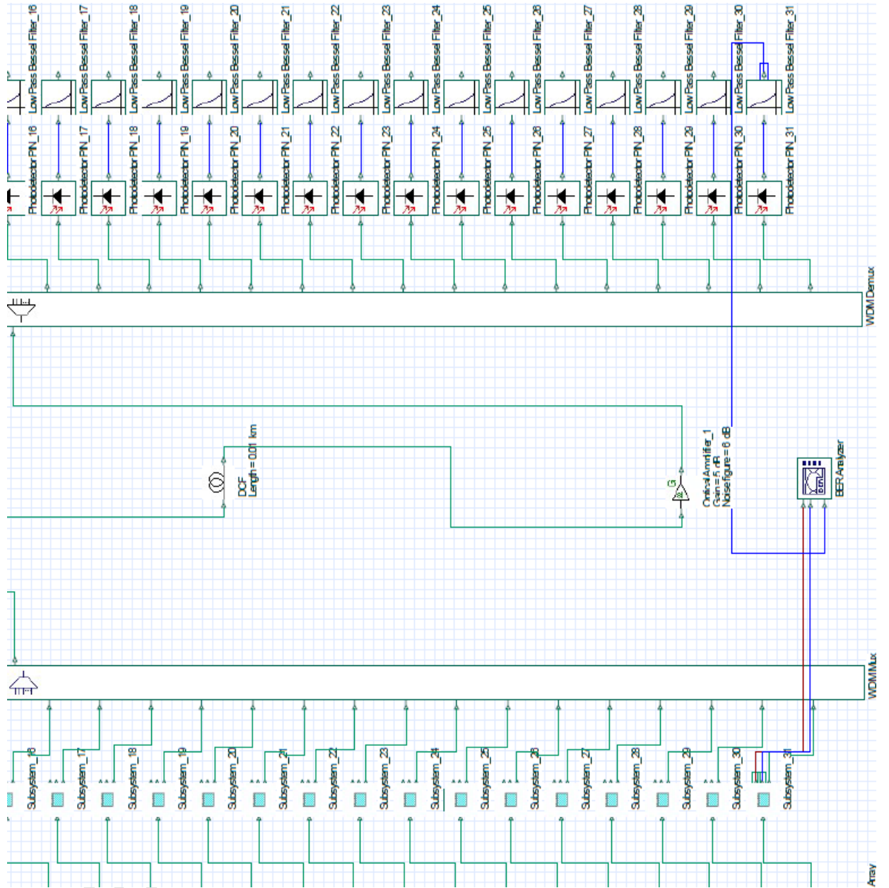
Figure 4: Simulation design of highly concentrated WDM (Wavelength division multiplexed) system
