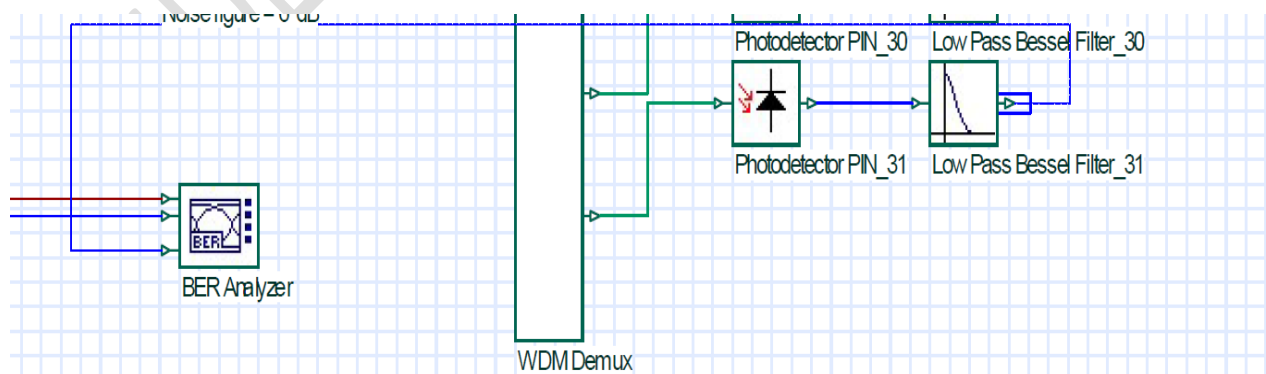
Figure 3: Design of receiver
