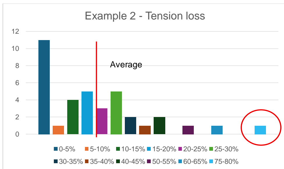
121 Figure 13 Tension loss less than 3 months after tensioning
