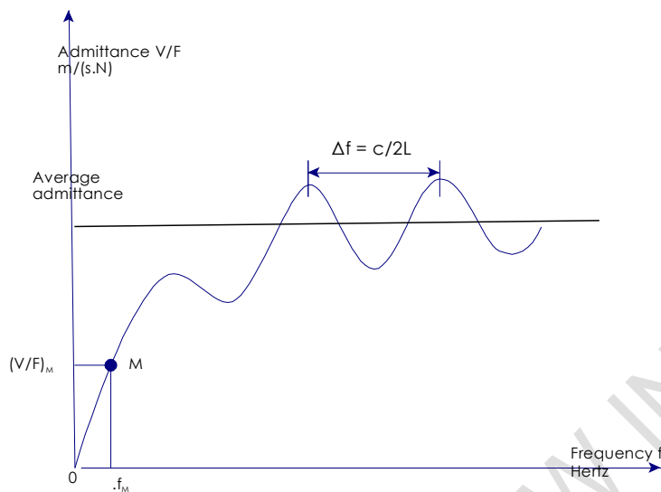
Figure 2 Velocity/Force as a function of frequency
