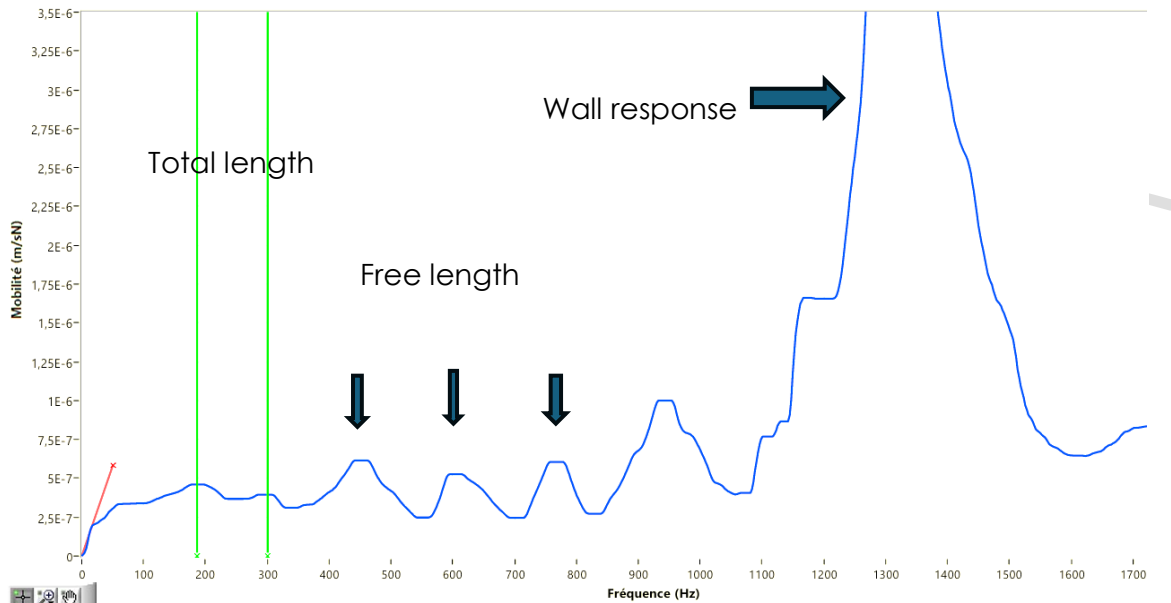
Figure 4 Typical response curve
