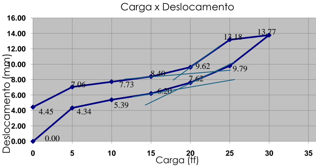
Figure 9 – Static test
