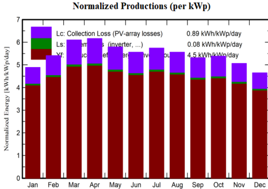
Figure 4: Normalized energy productions per installed kWp.
