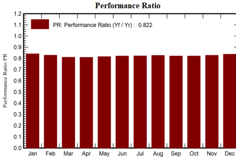
Figure 5: Performance ratio (%)
