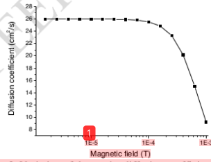
Figure 2. Variation of the carrier diffusion coefficient with magnetic field intensity.
