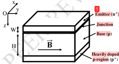
Figure 1. Simulated solar cell model.
