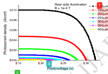
Figure 9: Photocurrent density as a function of photovoltage for various base thicknesses under rear-side illumination
