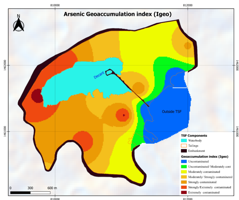
Figure 10: Spatial distribution of geo-accumulation indices for trace metals (As) in the tailings pond and surrounding soils
