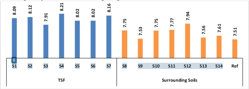
Figure 2: Variation in pH of mine tailings and surrounding soils
