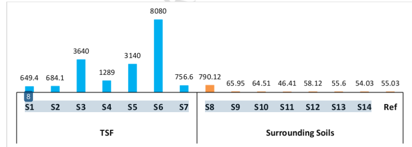
Figure 3: Surface dynamics of electrical conductivity (EC) in mine tailings and surrounding soils
