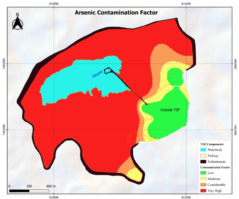
Figure 12: Distribution of the arsenic contamination factor in soils in and around the tailings facility
