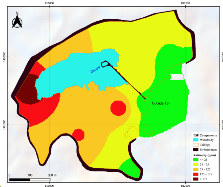
Figure 6: Spatial distribution of antimony contents in the tailings facility and surrounding soils compared to the local geochemical background
