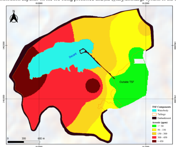
Figure 5: Spatial distribution of arsenic concentrations in the tailings facility and surrounding soils compared to the local geochemical background
