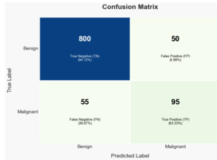
Fig. 7 Confusion Matrix
