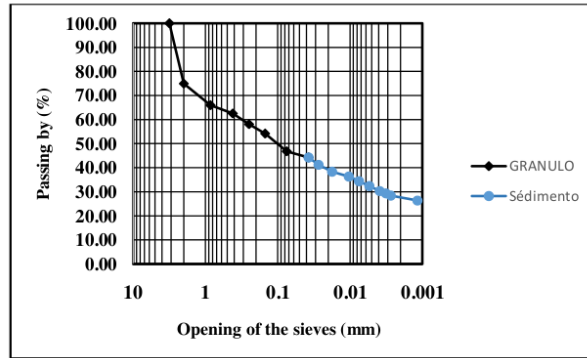
Figure1 : Granulometry and sedimentometry analysis
