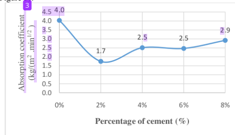
Figure 3: Change in capillary absorption coefficient
