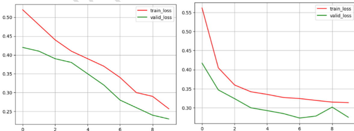
Figure 7: Training and validation loss of GPT and BERT in 10 epochs
