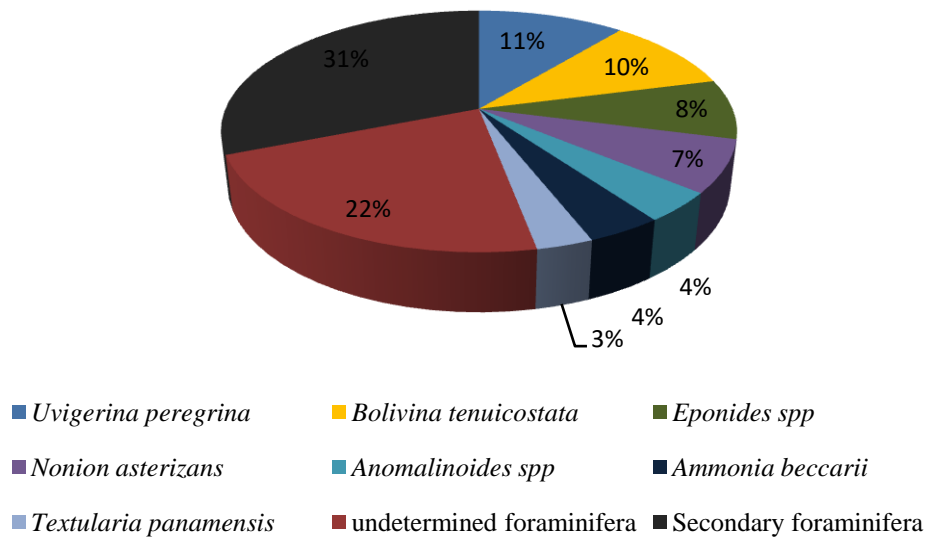
figure 6: distribution of calcareous benthic foraminifera
