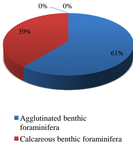
figure 4: distribution of benthic foraminifera
