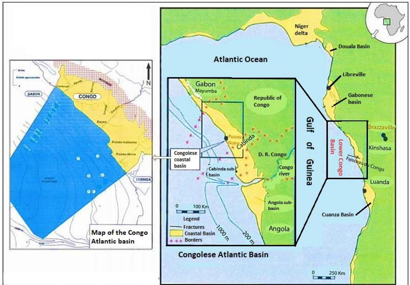
Figure 2: Location maps of the Congolese Atlantic basin (Vernet et al. , 1996)
