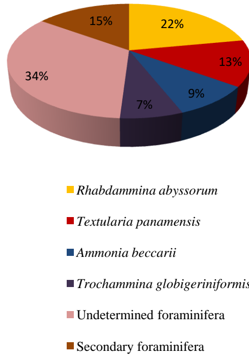
figure 5: distribution of agglutinated benthic foraminifera
