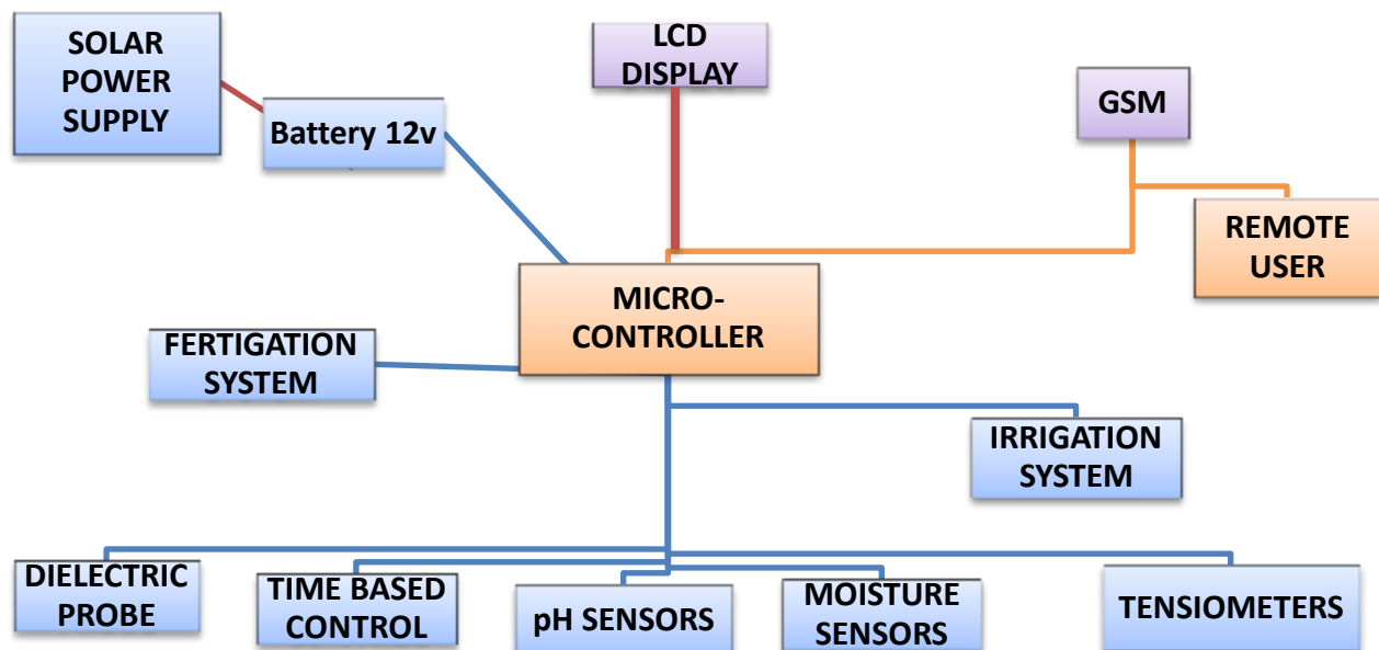
Figure 1:- System overview
