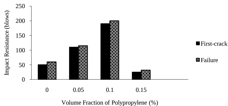
Figure 7: Effect of Polypropylene Fiber Addition on the Impact Resistance of SCC
