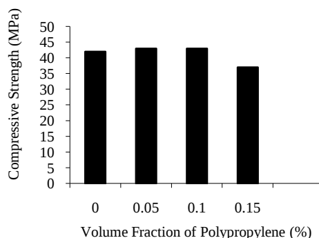
Figure 5: Effect of Polypropylene Fiber Addition on the Compressive Strength of SCC
