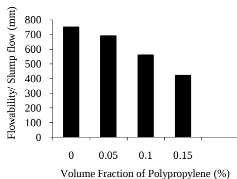
Figure 1: Effect of Polypropylene Fiber Addition on the Flowability of SCC Mixes
