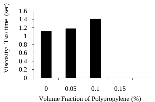
Figure 1: Effect of Polypropylene Fiber Addition on the Flowability of SCC Mixes
