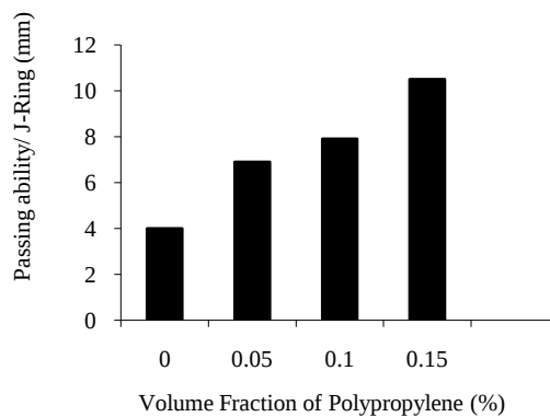
Figure 2: Effect of Polypropylene Fiber Addition on the Viscosity of SCC Mixes
