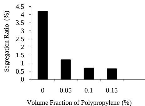
Figure 4: Effect of Polypropylene Fiber Addition on Segregation Ratio of SCC Mixes
