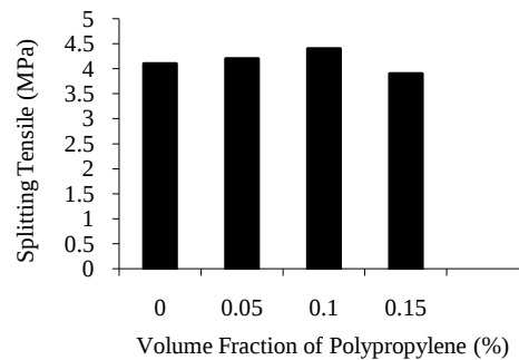
Figure 6: Effect of Polypropylene Fiber Addition on the Splitting Tensile Strength of SCC
