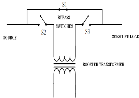
Figure2: Protection mode of a DVR
