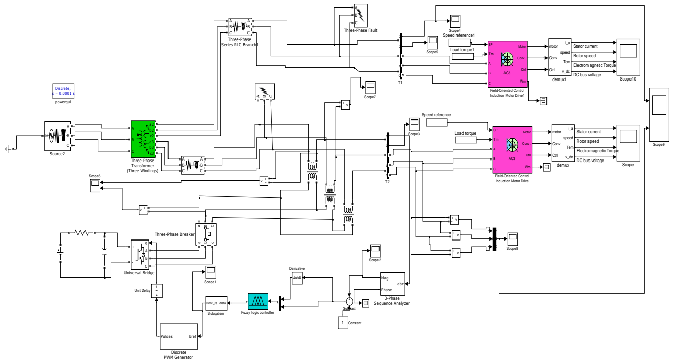
Figure8b: Simulation Model of DVR Test System
