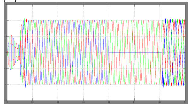
Figure9(a): Output load voltage of SLGFault without compensation
