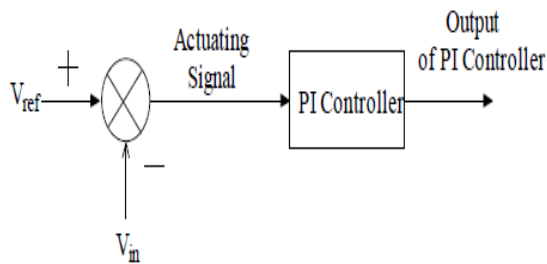
Figure4: Schematic of a typical PI Controller
