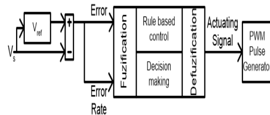
Figure6: Block diagram of proposed control system
