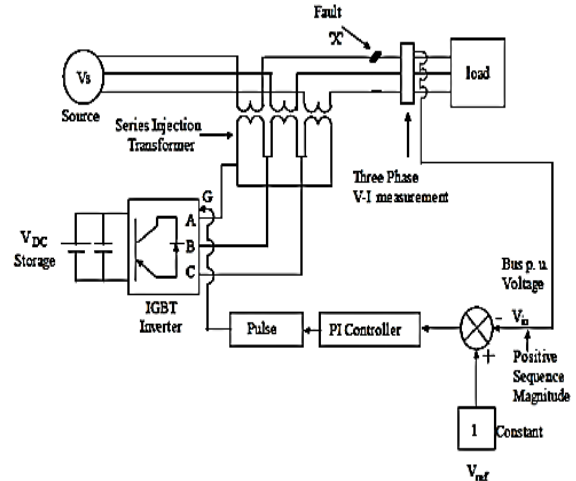
Figure5: Circuit Model of DVR Test System
