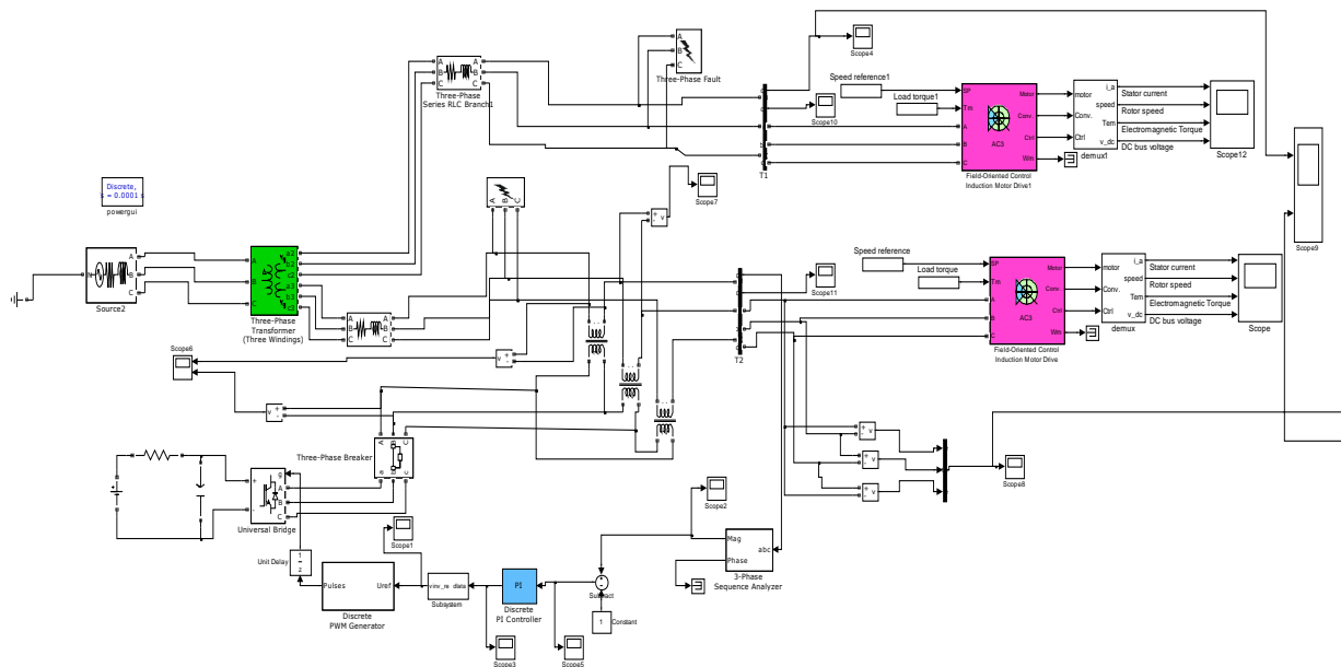
Figure8a: Simulation Model of DVR Test System
