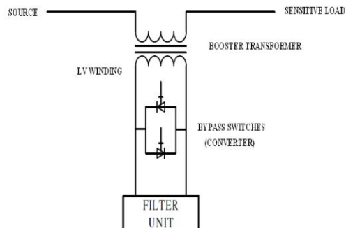
Figure3: Standby mode of a DVR
