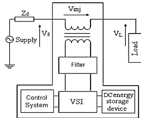
Figure1: Schematic representation of a DVR
