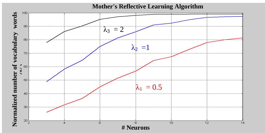
Figure 4: Graphical simulation results obtained for 'reached vocabulary number of words' versus different gain factor values ( \lambda_1 , \lambda_2 , and \lambda_3 )=(0.5, 1, and 2) ; while # Neurons increases.
