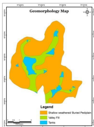
Fig.7. Geomorphology map
