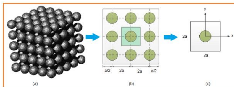
Figure 1: A square RVE containing a nanoparticle.
