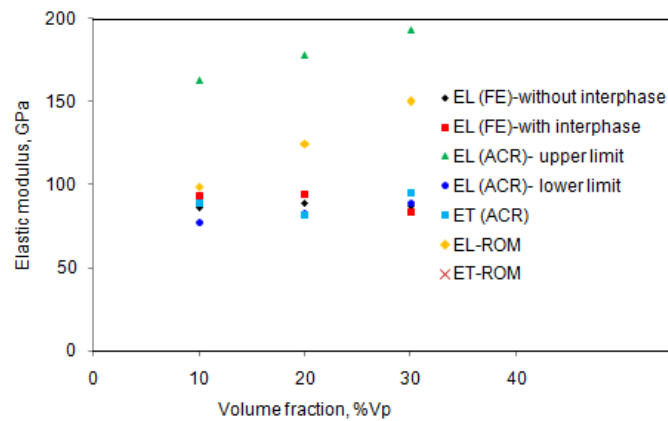
Figure 6: Elastic moduli of AA3105/AlN nano composite.
