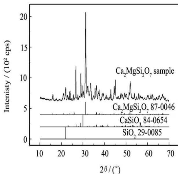
Fig.1 XRD pattern of \text{Ca}_2\text{MgSi}_2\text{O}_7 ; \text{Dy}^{3+} (4mol%)
