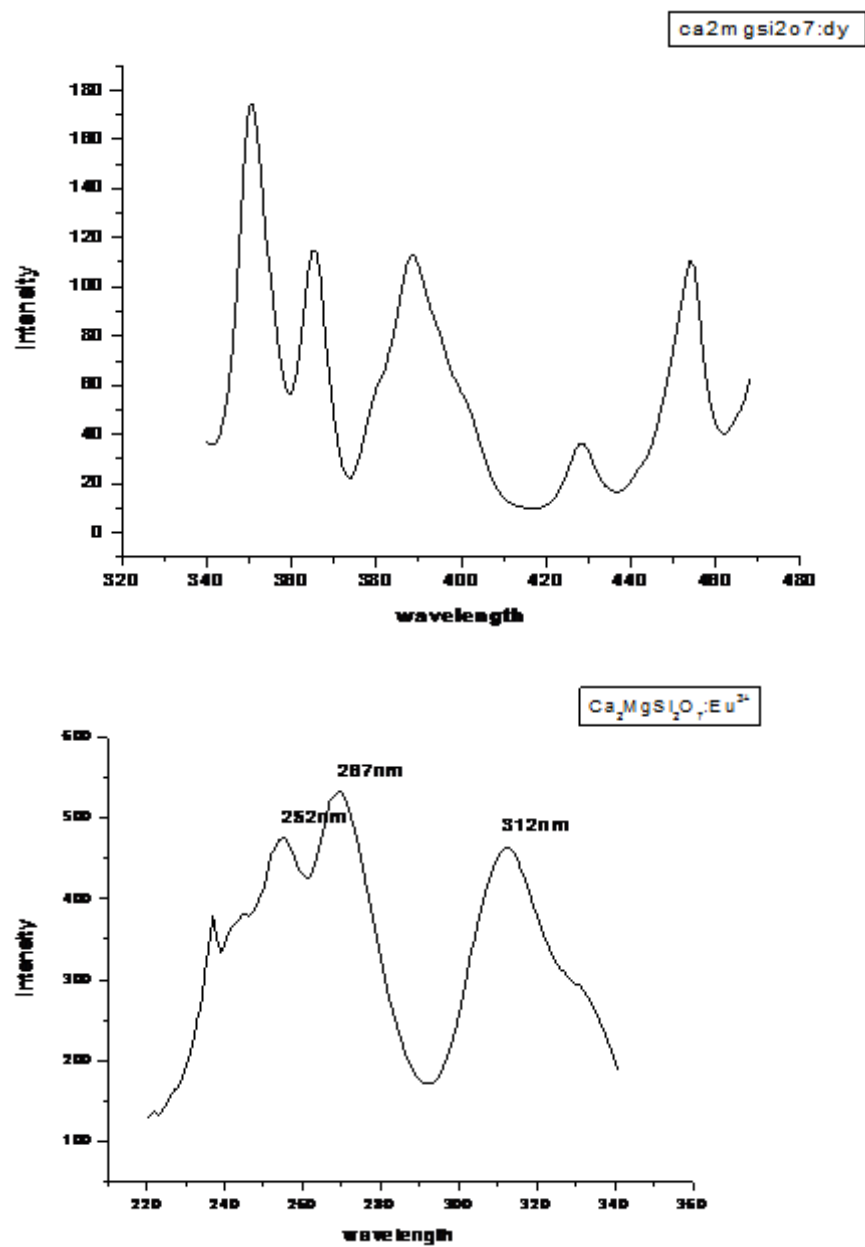
Fig2(a) Excitation Spectra of \text{Ca}_2\text{MgSi}_2\text{O}_7:\text{Dy}^{3+} ( \lambda_{\text{em}}=481\text{nm} ) and fig (b) Excitation Spectra \text{Ca}_2\text{MgSi}_2\text{O}_7:\text{Eu}^{2+} ( \lambda_{\text{em}}= 615\text{nm} ).
