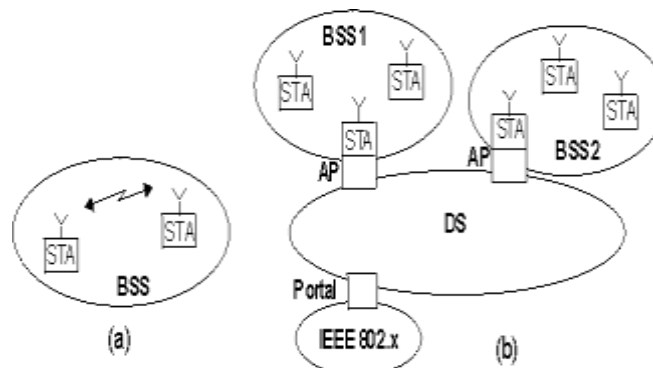
Figure 11:- Example of infrastructure network
