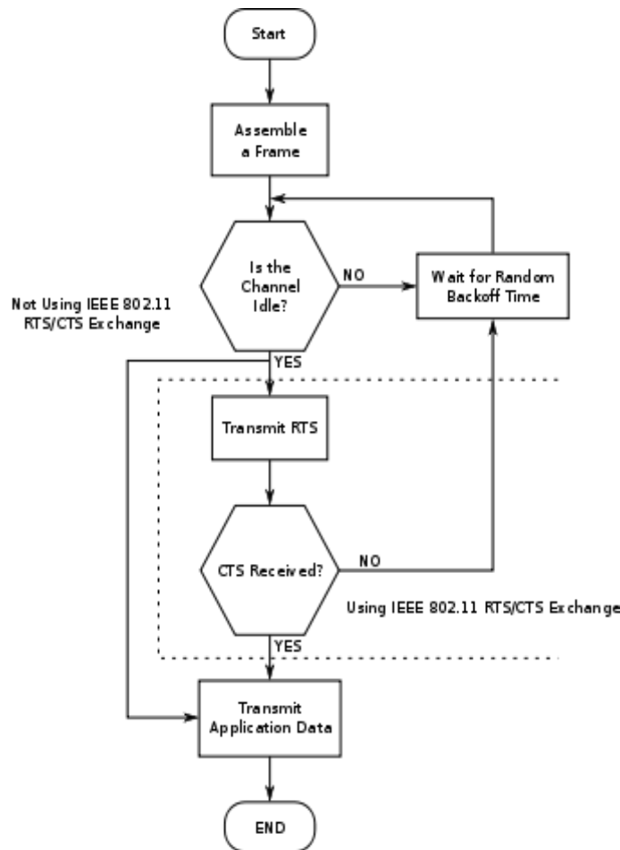
Figure 4:-Flow chart of CSMA/CA
