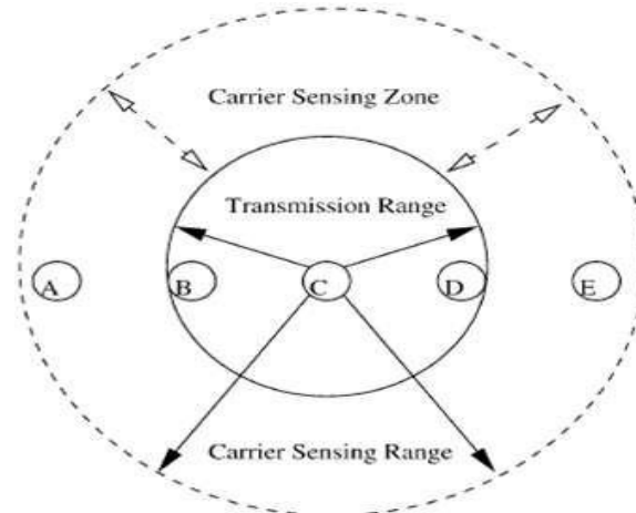
Figure 9:-Carrier Sensing
