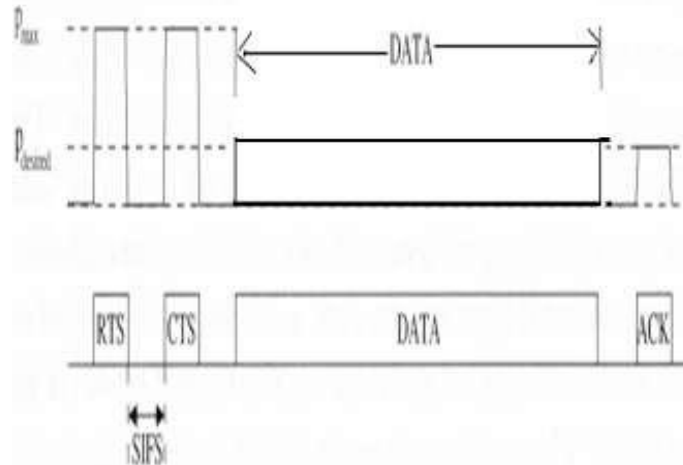
Figure 15:-Basic Power Control Protocol.
