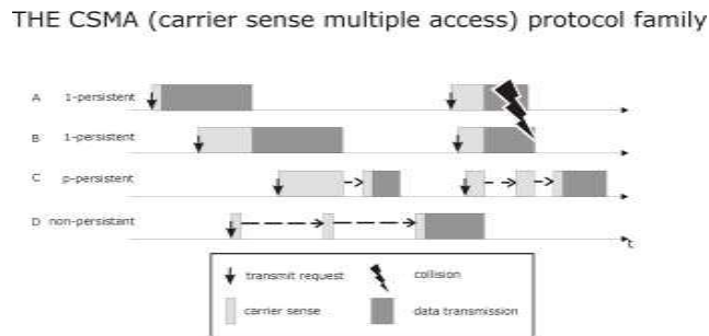
Figure 3:- CSMA Channel Access Mechanism
