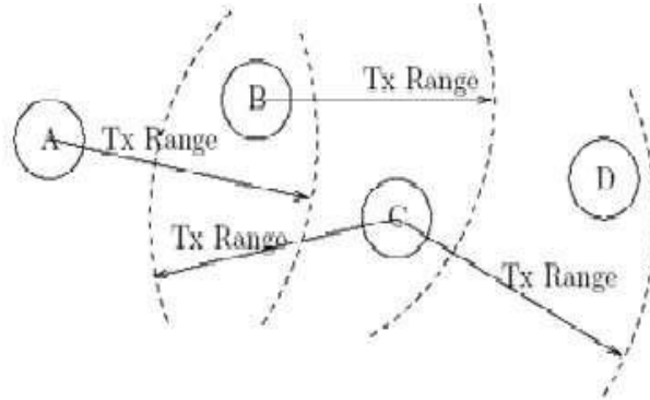
Figure 2:- Hidden & Exposed node problem
