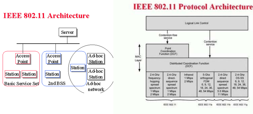
Figure 8:-IEEE 802.11 Protocol Architecture
