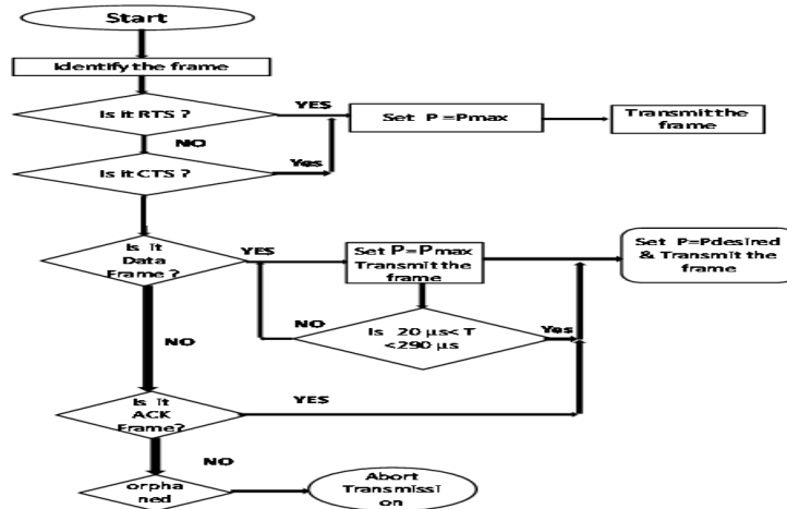
Figure 18:-Flow chart of Proposed Protocol
