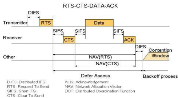
Figure 13:-NAV duration in transmission range and carrier sensing zone
