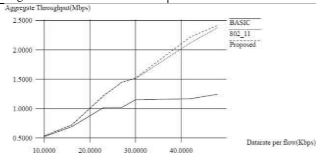
A. Simulation Result for Aggregate Throughput vs Data Rate Per Flow
