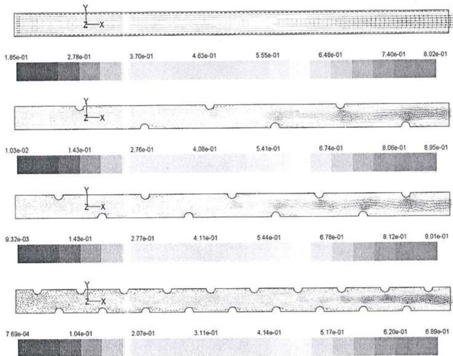
Figure (6):- Speed distribution at Re = 500 and (Q = 3000) .
