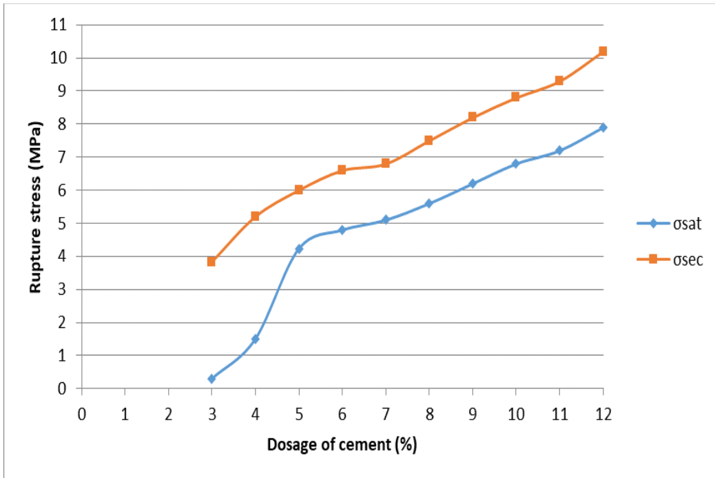
Fig. 16:- Variation of the \sigma_{sat} and \sigma_{dry} as a function of dosage of cement.
