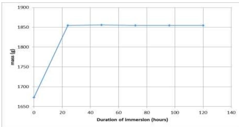
Fig. 10:- Curve of variation of the mass of the immersed bricks as a function of time.
