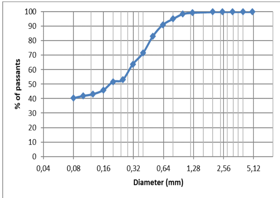
Fig. 9:- Granulometric curve of the soil.
