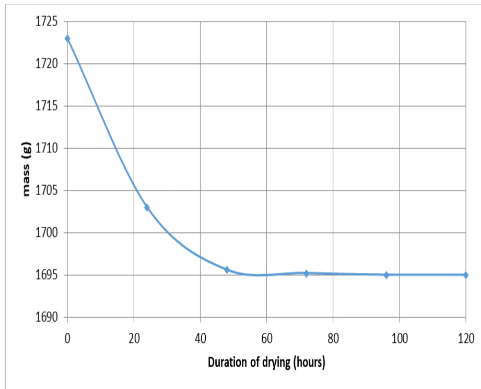
Fig. 11:- Curve of variation of the mass of the dry bricks as a function of time.
