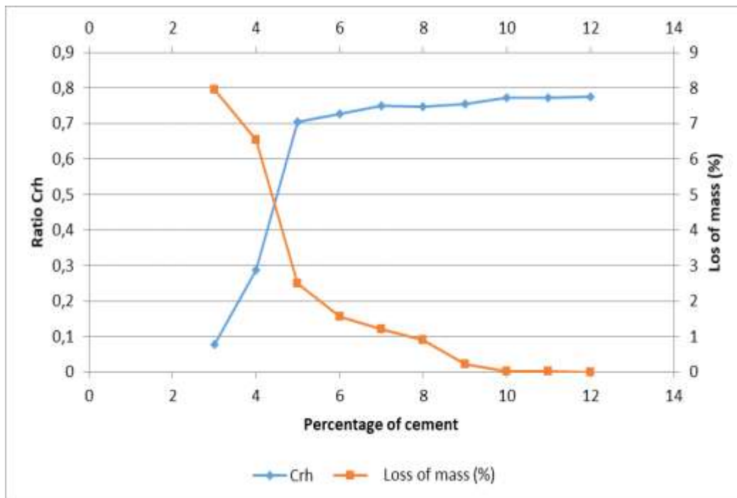
Fig. 17:- Variation of C_{rh} and loss of mass as a function of dosage of cement.
