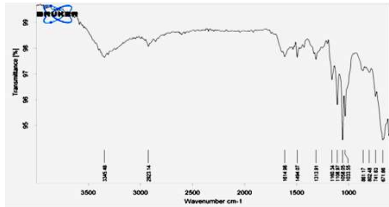
Figure 5: FTIR Spectra of PANI/BC Composites.
