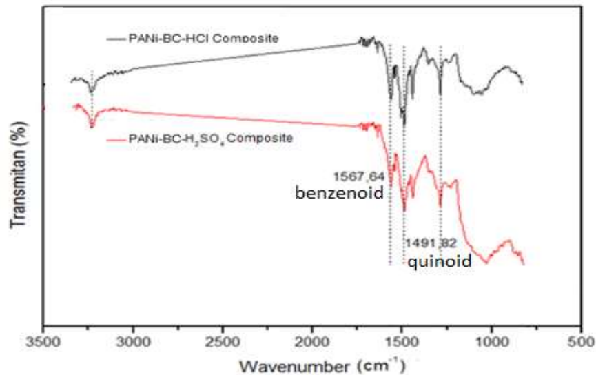
Figure 6: FTIR spectra of polyaniline and PANI-BC composites.
