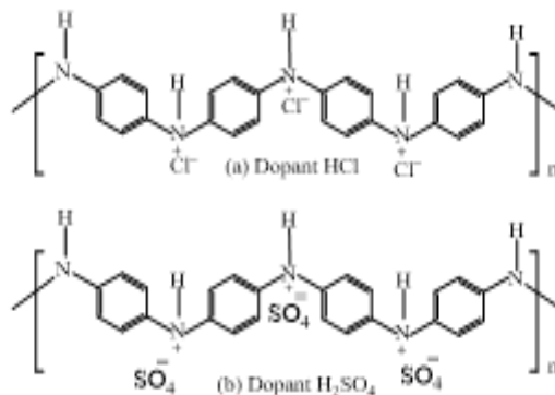
Figure 3:- Struktur Polianiline Garam Emeraldine (a) Dopant of HCl; (b) Dopant of H_2SO_4
