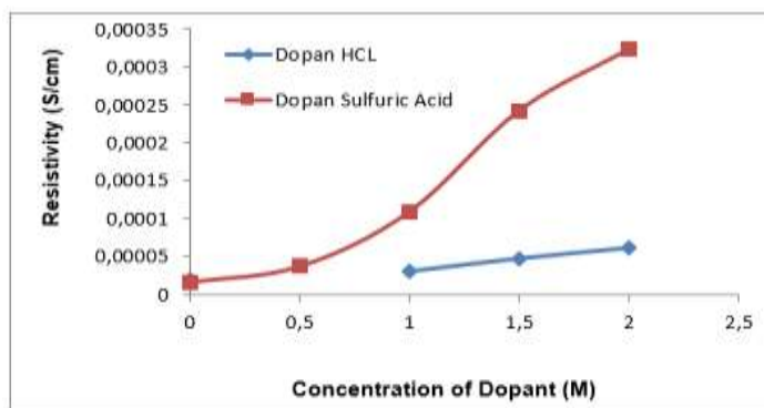
Figure 7: The conductivity of PANI-BC/HCl and PANI-BC/H 2 SO 4 composites.
