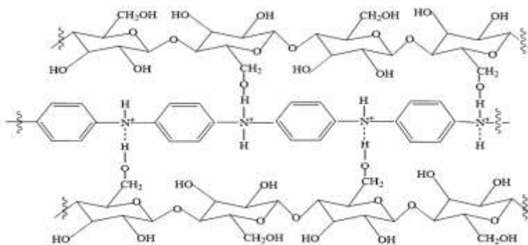
Figure 1:- Polyaniline-BC dopant HCl conductive composite models.
