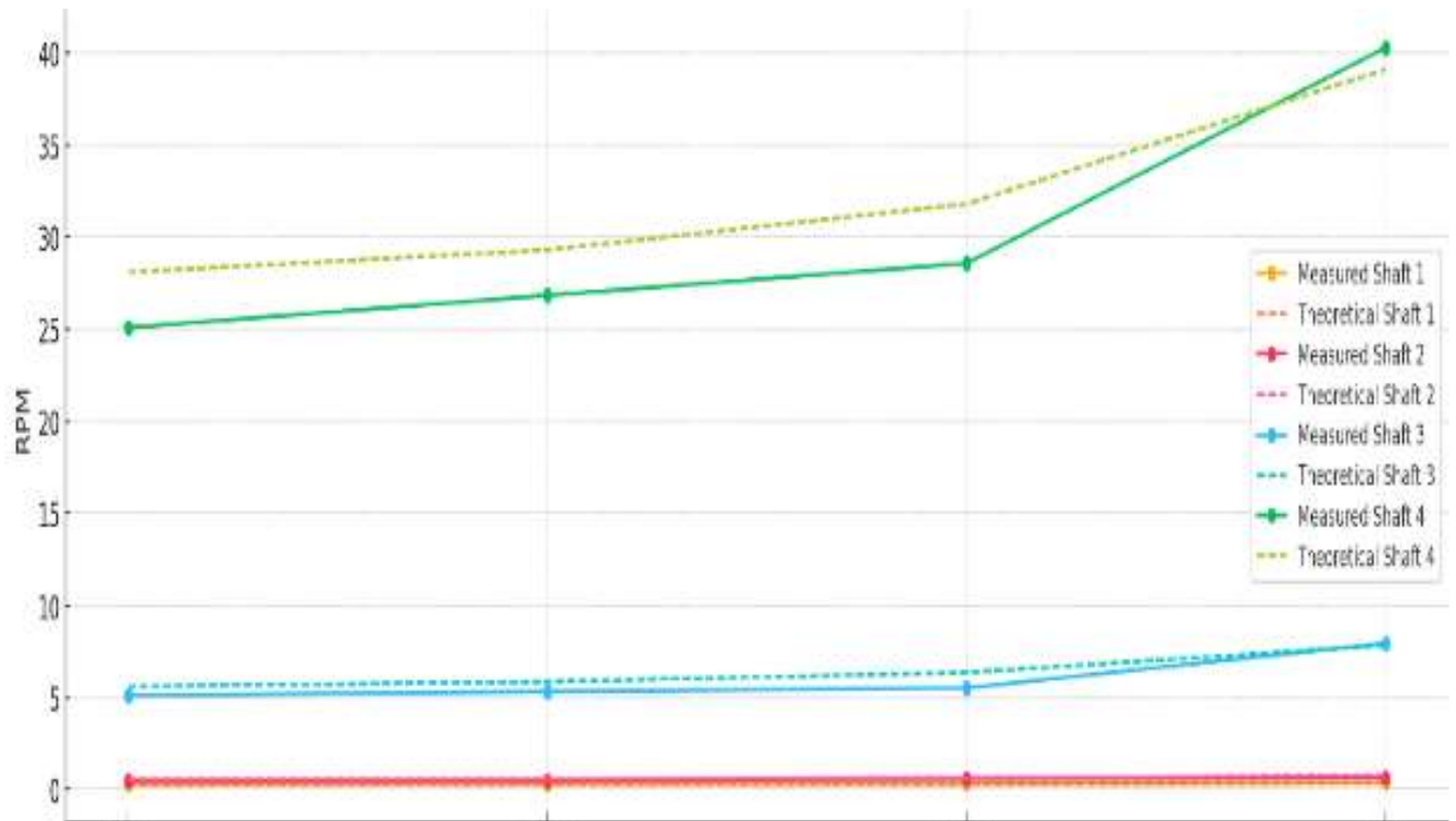
Figure 1:- Comparison of Measured Vs Theoretical RPM per Shaft.
