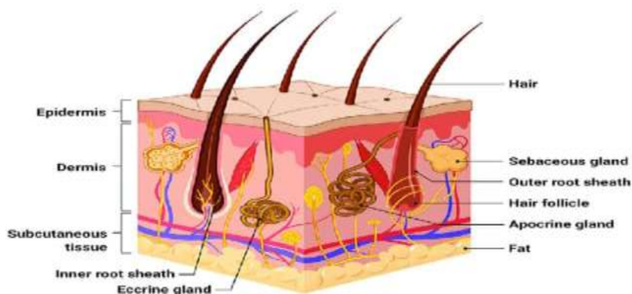
Figure1:-Skin's structure
