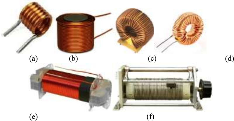
Figur 2.2 a,b,c,d,e,f Inductor Components:
