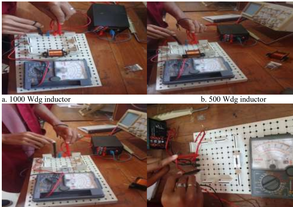
c. 33 mH inductor
