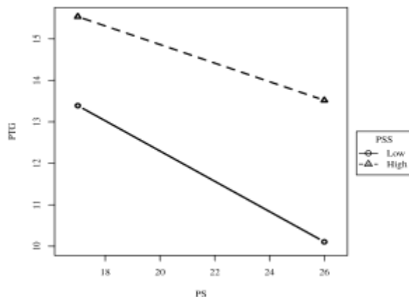
Figure 3 : Regression lines for PTG predicted by PS for the High and Low categories of PSS
