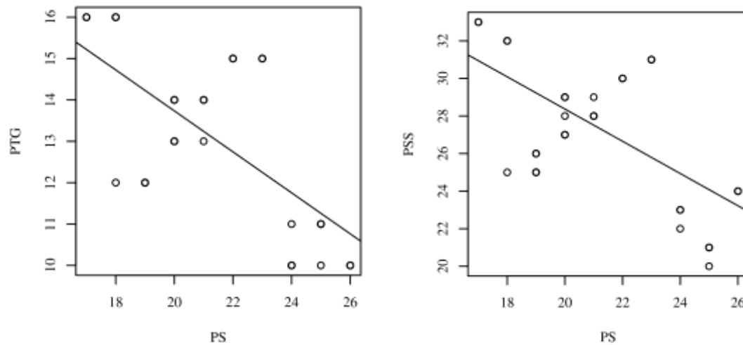
Figure 2 : Scatterplots with the regression line added for PTG and PSS
