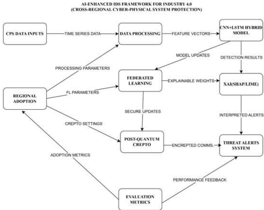
Figure 1: Framework design for cross-regional CPS Security
