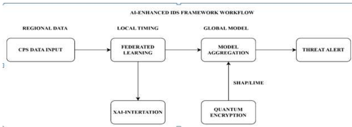
Figure 2: Conceptual diagram workflow of AI-Enhanced Intrusion Detection System (IDS) framework
