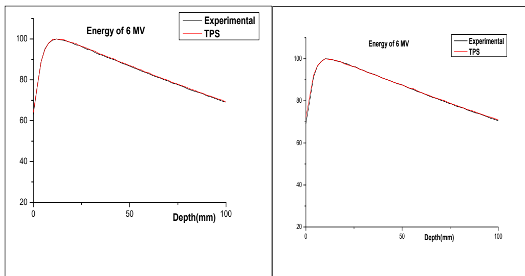
Fig.1. comparison of measured and calculated results of percentage depth dose curves of the 6MV photon beam. Fig. (a) is for field size 10 cm \times 10 cm, (b) is for 20 cm \times 20 cm.(c) is for 30 cm \times 30 cm , (d) is for 40 cm \times 40 cm.
