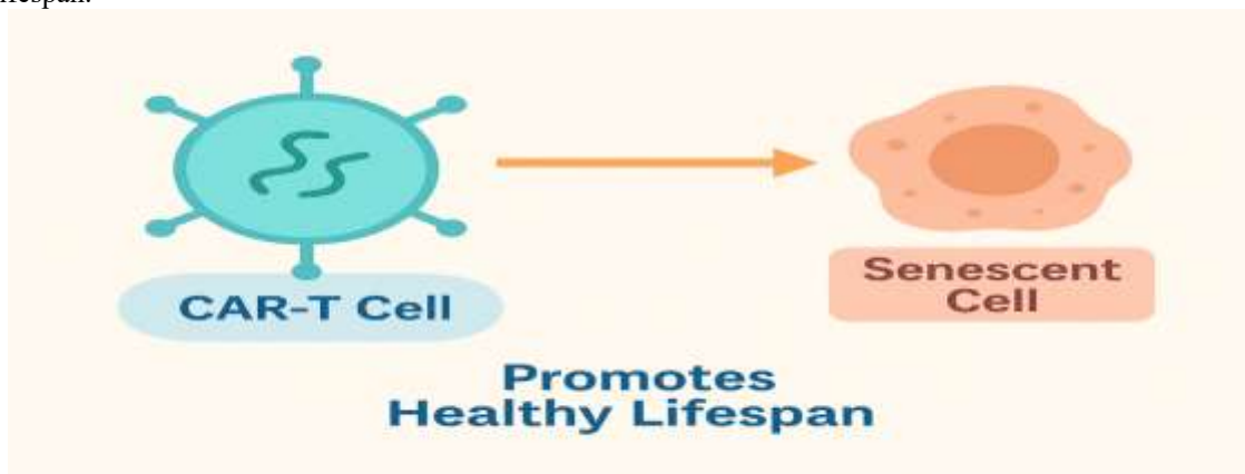
Fig.5: CAR-T Cells Targeting Senescent Cells
