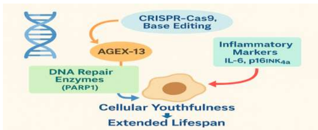
Fig. 3: CRISPR-Cas9 and Base Editing Simulations
