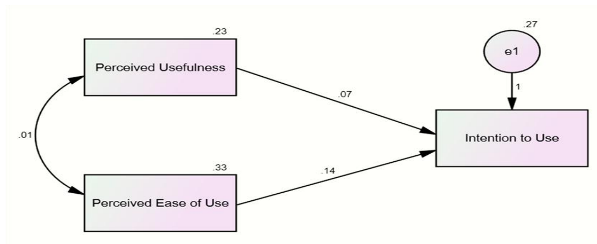
Fig 1 : Structural Equation Modeling
