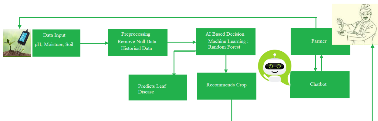
Figure 6: System Architecture
