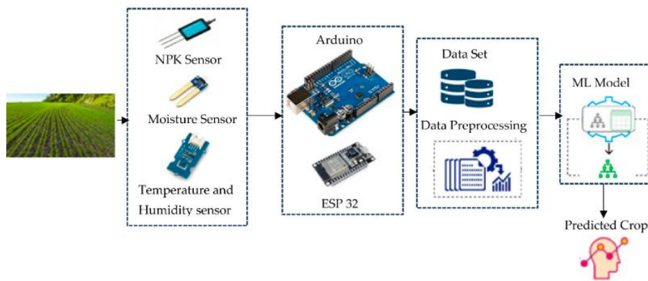
BLOCK DIAGRAM FOR REAL TIME CROP ADVISORY SYSTEM
