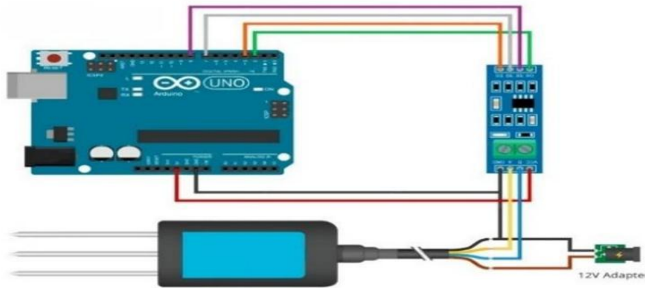
Figure-5: Arduino – NPK interfacing:
