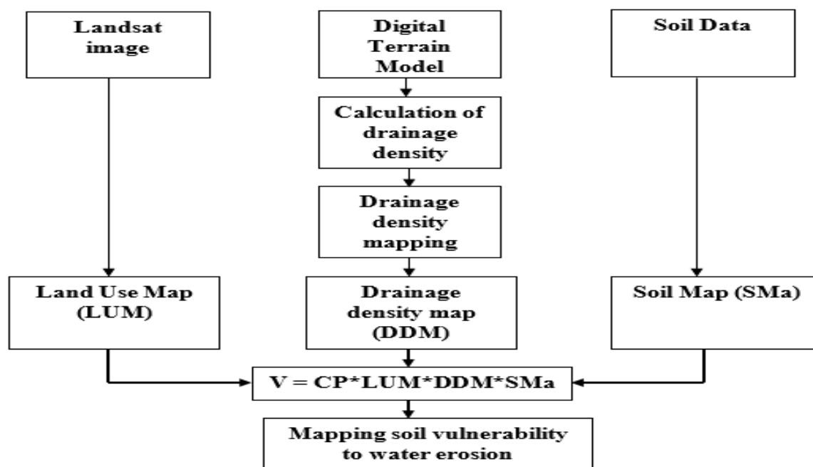
Figure 2: Methodology for mapping soil vulnerability to water erosion in the Agneby watershed
