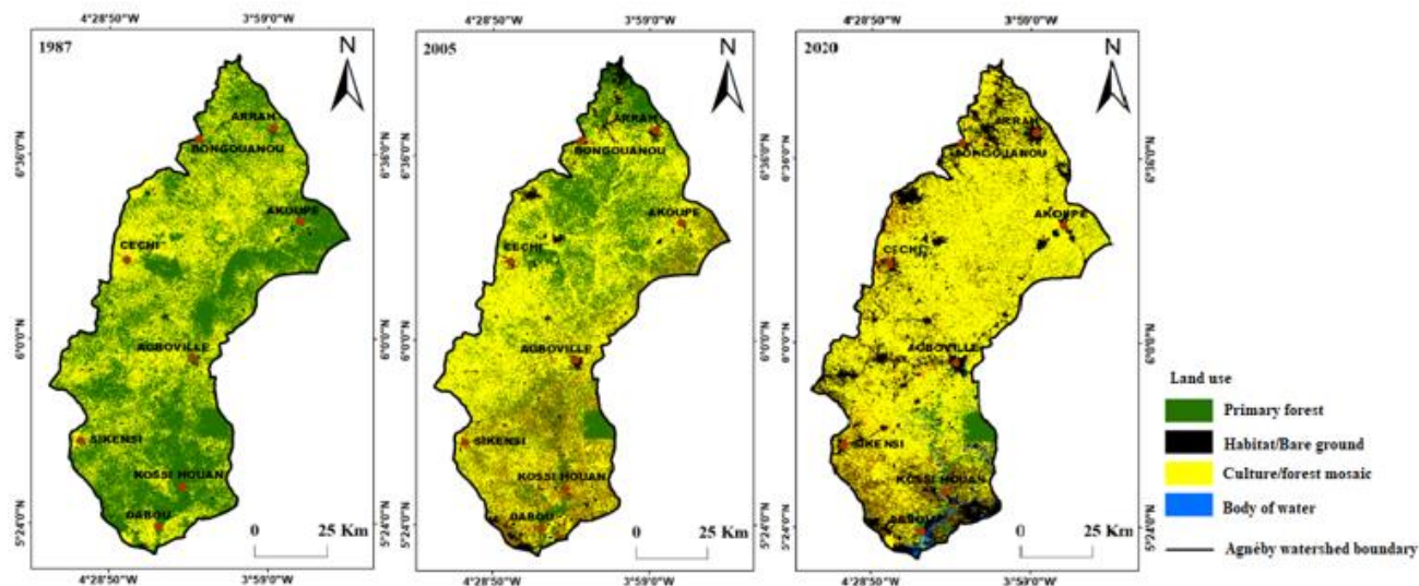
Figure 3: Land use from 1987 to 2020 in the Agneby watershed
