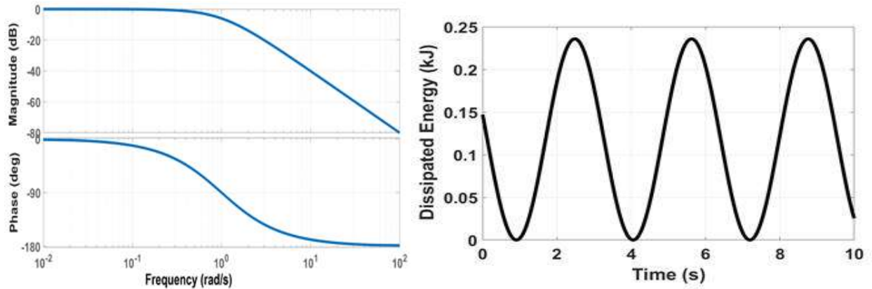
Figure 8: Left: Frequency Response Analysis. Right: Energy Dissipation Over Time.
