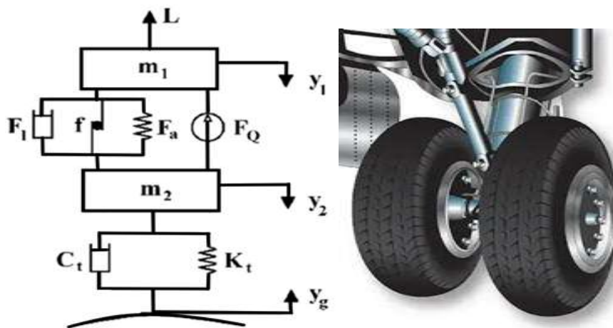
Figure 1: Schematic of landing gear.
