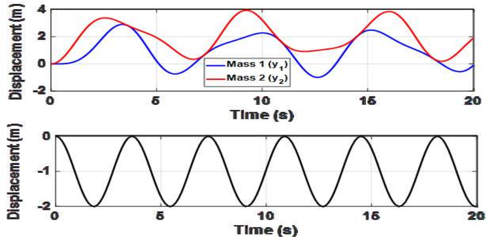
Figure 5: Displacement of masses (above), and relative displacement between the masses (below).
