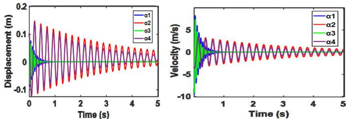
Figure 6: Displacement (left) and Velocity (right) for Different Mass (m), Stiffness (k), and Damping (c) with the proposed FOPID controller.
