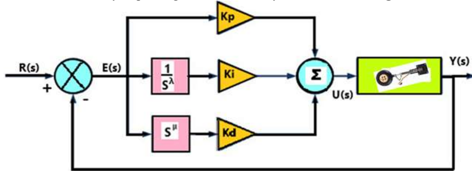
Figure 2: Proposed FOPID controller diagram
