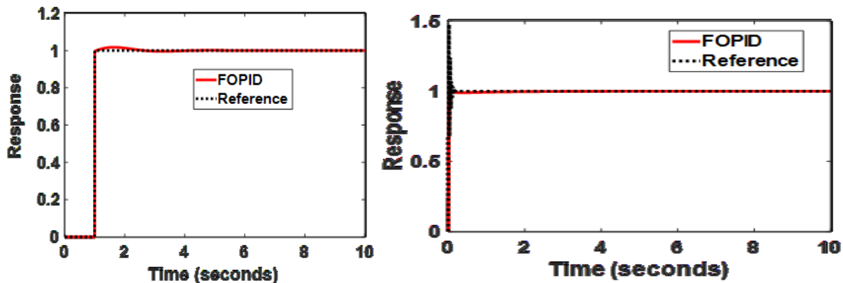
Figure 4: FOPID Controller step (left) and non-step (right) response plots.
