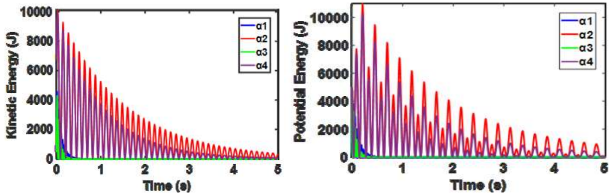
Figure 7: Kinetic Energy (left) and Potential Energy (right) for Different Masses
