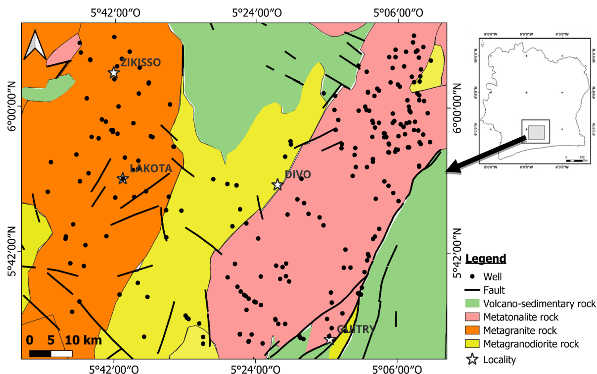
Figure 1. Map presenting the study area and distribution of lithological formations (modified from Delor et al., 1995)
