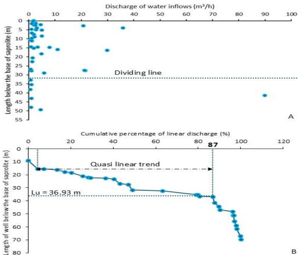
Figure 5. Vertical distribution of the properties of the MGDR aquifer: a) analysis with inflows; b) analysis with cumulative percentages
