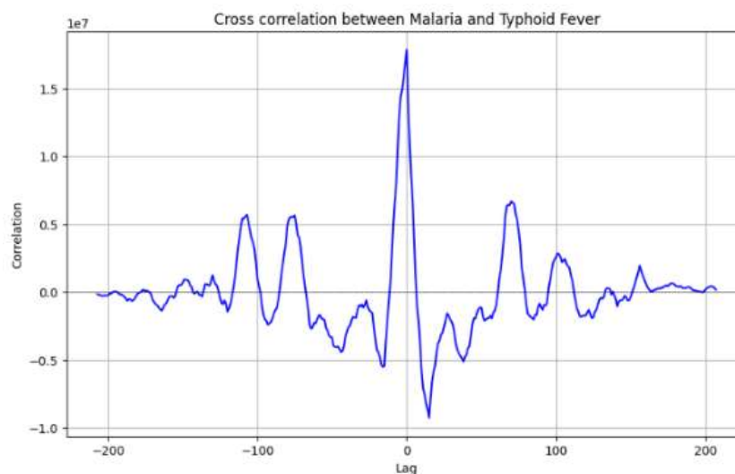
Figure 4: Cross-correlation
