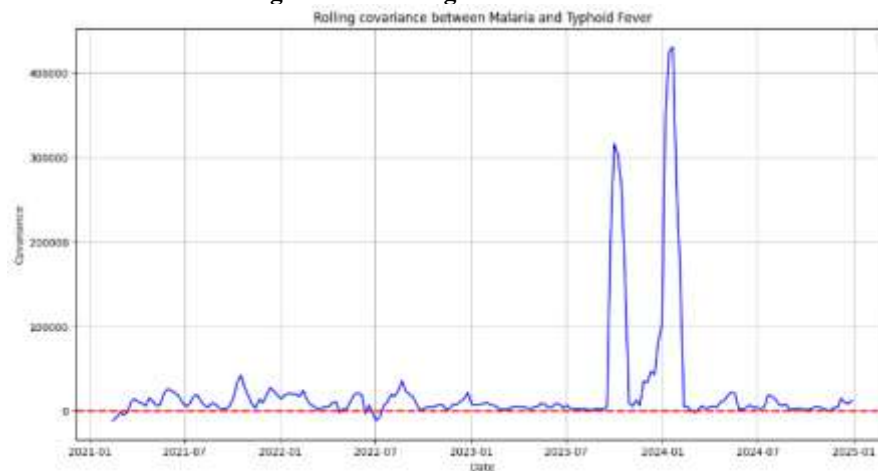
Figure 9: Rolling covariance
