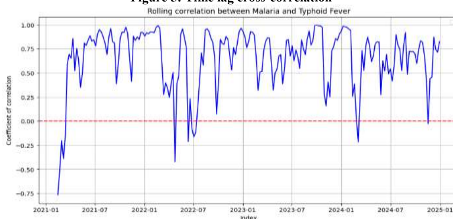
Figure 6: Rolling correlation
