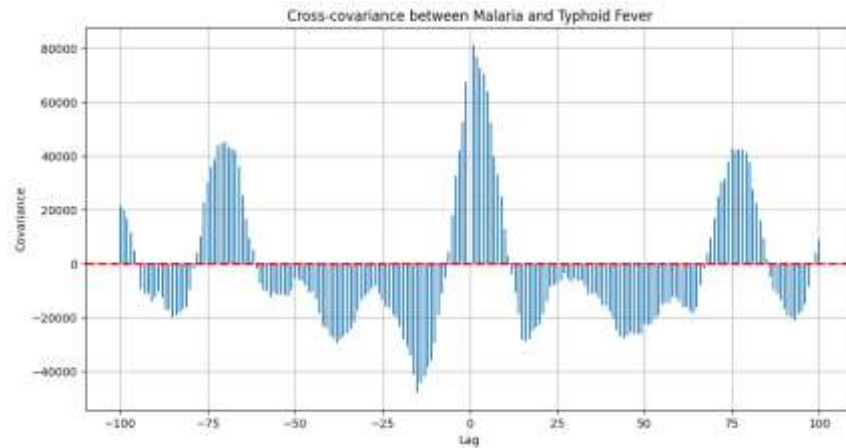
Figure 7: Cross-covariance
