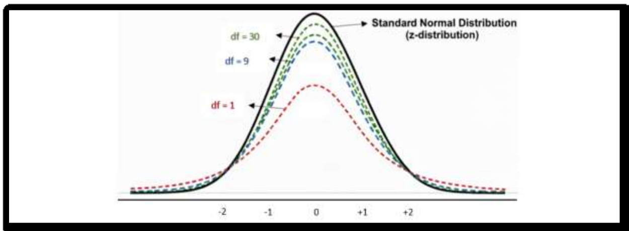
Figure 2: z-distribution vs. t-distribution
