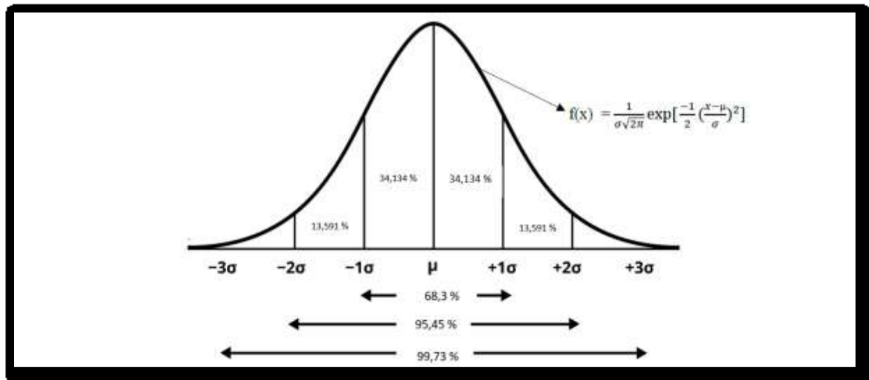
Figure 3: Coverage Probabilities
