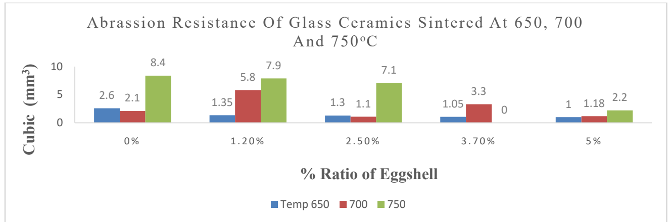
Figure 18: Abrasion Resistance of the Sintered Glass ceramics
