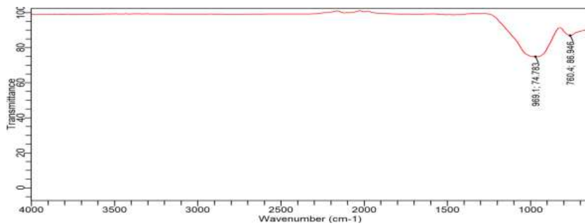
Figure 4: FT-IR of Waste Glass Powder
