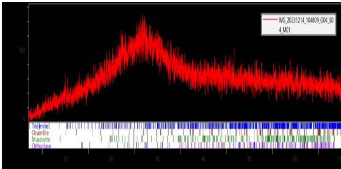
Figure 2: X-ray Diffraction of Glass Powder
