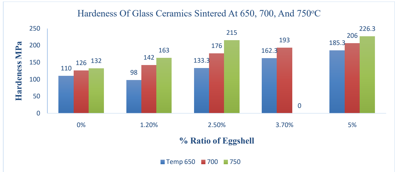
Figure 14: Hardness of the Sintered Glass Ceramics
