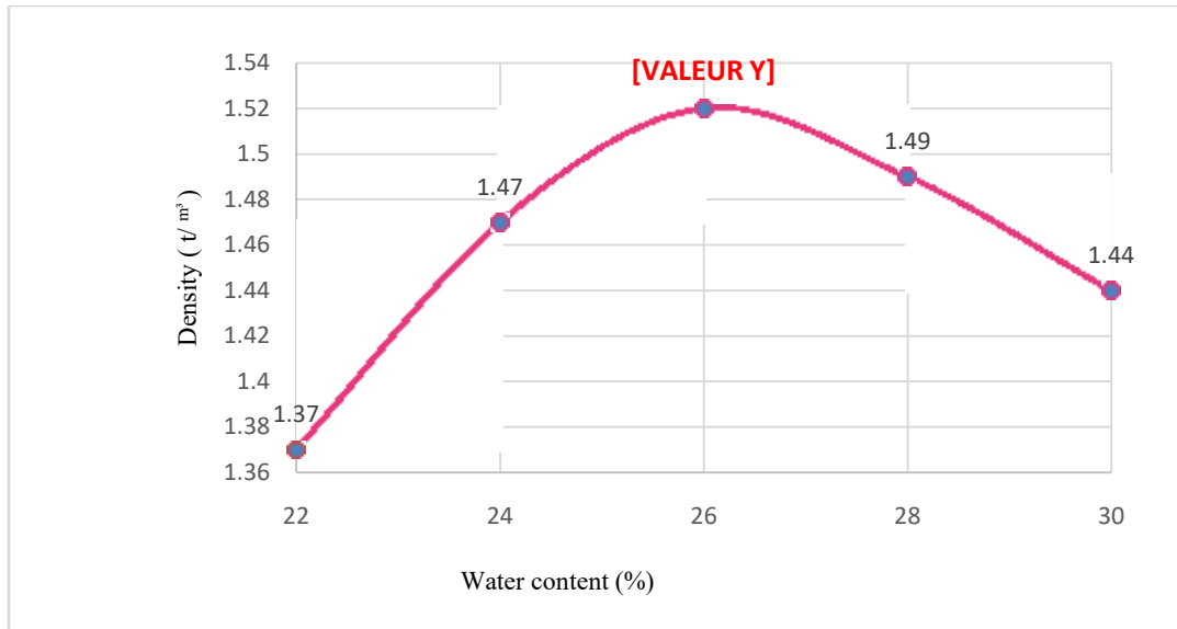
Figure 4: Modified Proctor curve of the studied clay
