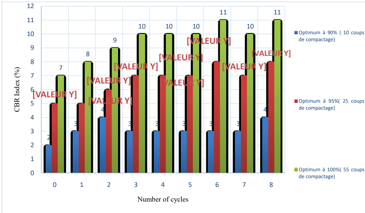
Figure 5: Variation of the soil CBR index as a function of the wetting-drying cycle
